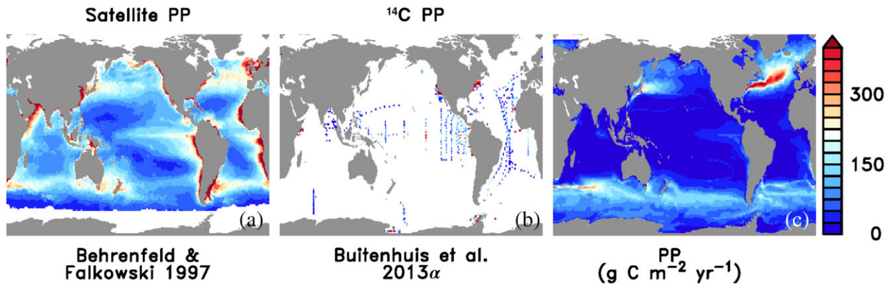
Fig. 5. Observed NPP from satellite observations (a) and oceanic measurements of ^{14}\text{C} NPP (b) compared to PP simulated with the standard configuration (c).
