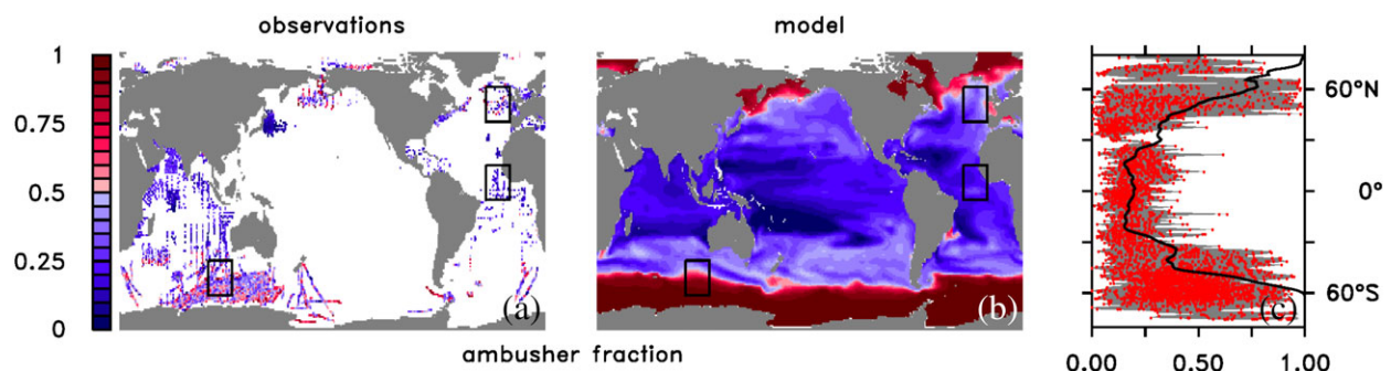
Fig. 2. (a) Observed ambusher fraction of total copepods at all stations where Oithona spp. as proxy for ambushing copepods was identified. (b) Simulated annual average ambusher fraction. (c) The zonal average of the simulated ambusher fraction (black line) together with all observational data points shown in panel a (red dots), gray shading indicates the range of observations. All data are averages from 0 m to 100 m depth. Boxes in panels (a) and (b) indicate the locations examined in Fig. 6.
