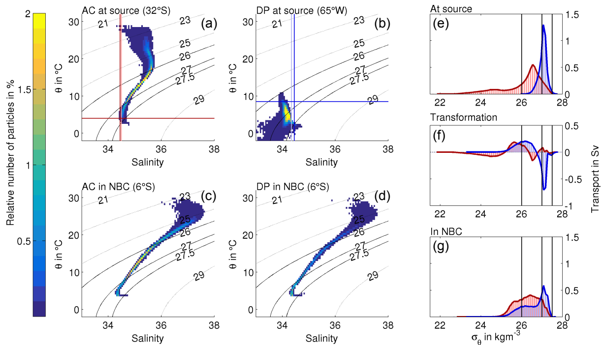
Figure 7. Mean potential temperature ( \theta ) and salinity ( S ) characteristics, as well as transformation in density space of waters with AC and DP origin. (a-d) Relative number of particles from all 10 REF experiments per 0.5\text{ }^{\circ}\text{C} \times 0.1\text{ psu} bin, i.e., local count divided by the total number of released particles in the respective subset, in %. (e-g) Mean volume transport per density class (in 0.1\text{ kgm}^{-3} bins) at source regions and in NBC, as well as volumetric water mass transformation (red: waters of AC origin, blue: waters of DP origin). Potential density levels used to separate surface, central, intermediate (and deep) waters are highlighted by solid black lines; dark blue (dark red) lines mark T and S values that constitute the upper (lower) limit for 99 % of the DP (AC) water volumes, light blue (light red) lines the respective limit for 95 %.
