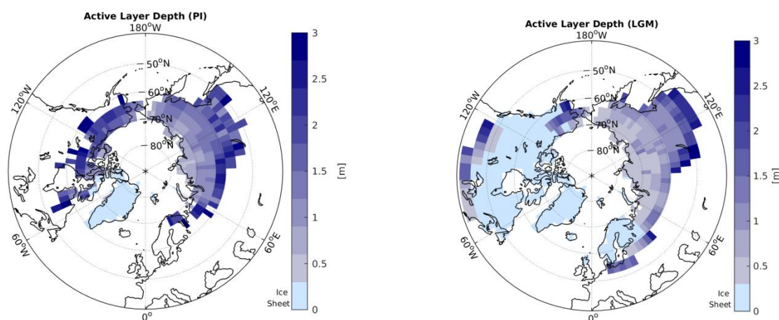
20 Figure 3: Active layer depths in near-surface permafrost soils at PI and LGM simulated by JSBACH. Light bluish areas show prescribed ice sheet coverage. Data shown represent hundred year time averages.
