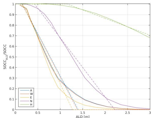
5 Figure A11: Dependency of vertical soil carbon concentration at the permafrost table on active layer depth (ALD) as simulated by the process-based SOM transport model. The ratio of equilibrium SOCC at the active layer depth SOCC_{AL}^i to mean seasonally thawed SOCC^i is shown for individual soil carbon liability pools. Values smaller than one are indicative of SOCC declining with depth. Dotted lines illustrate linear approximations used for implementation into JSBACH. Curves are inferred for default parameters of the process-based SOM transport model (cryoturbation rate: 10 \text{ cm}^2 \text{ yr}^{-1} , sedimentation rate: 10 \text{ cm kyr}^{-1} , litter input described by grassland).
