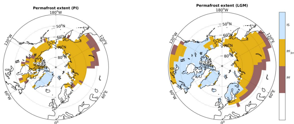
20 Figure 2: Ice sheet coverage and permafrost extent at PI and LGM simulated with JSBACH. Mustard areas illustrate grid cells of simulated near-surface permafrost with active layers above three meters (PF 3m ), brown-mauve areas describe permafrost with active layers deeper than three meters (PF). Light bluish areas show prescribed ice sheet coverage (IS). Data shown represent hundred year time averages.
