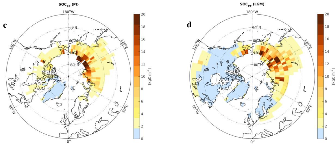
5 Figure 5: Seasonally thawed SOC in the active layer ( SOC_{AL} - panels a,b) and perennially frozen SOC in near-surface permafrost ( SOC_{PF} - panels c,d) at PI and LGM simulated by JSBACH. Light bluish areas show prescribed ice sheet coverage. Data shown represent hundred year time averages.
