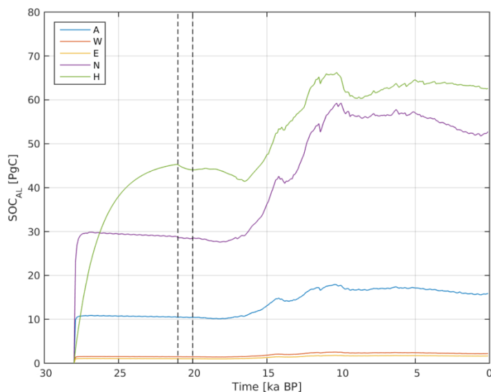
Figure A12: Simulation set-up for deglacial model runs. Shown is the spinup and fully transient phase of active layer SOC pools for all SOM lability classes (A, W, E, N, H) from the experiment initialization at 28 ka BP to 0 BP. The vertical dashed line at 21 ka BP illustrates the end of the SOC spinup phase, the vertical dashed line at 20 ka BP illustrates the end of the stationary LGM climate forcing.
