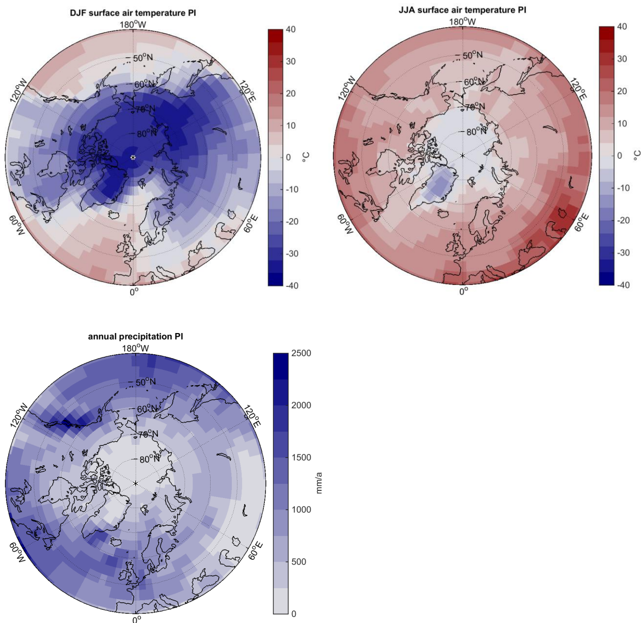
Figure A3: PI winter surface air temperatures (DJF), summer surface air temperature (JJA) and annual precipitation simulated by MPI-ESM_1.2T31_PI.
