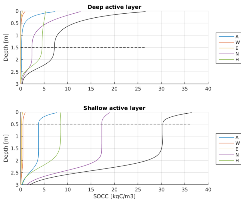
15 Figure A10: Simulated SOCC profiles inferred from the process-based model of vertical SOM dynamics. The coloured curves represent different SOM lability classes according to YASSO, separated into fast (A,W,E), intermediate (N), and slowly decomposing (H) compounds. The black line shows aggregated total SOC. The horizontal dashed lines indicate active layer depth, and determine SOCC_{AL}^i . Simulations were run for 20 kyrs using a cryoturbation rate of 10 \text{ cm}^2 \text{ yr}^{-1} , a sedimentation rate of 10 \text{ cm kyr}^{-1} , decomposition timescale parameters set to YASSO standard values, and using a litter input of 100 \text{ gC yr}^{-1} \text{ m}^{-2} (upper panel) and 200 \text{ gC yr}^{-1} \text{ m}^{-2} respectively (lower panel).
