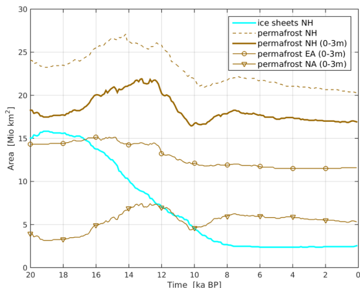
5 Figure 6: Deglacial evolution of simulated permafrost extent and prescribed ice sheet area from LGM to PI. Permafrost extent (brown lines) is shown separately for total (dashed line) and near-surface (solid line) northern hemisphere permafrost, subdivided into North America (triangled line), and Eurasia (circled line). Data shown represent hundred year time averages.
