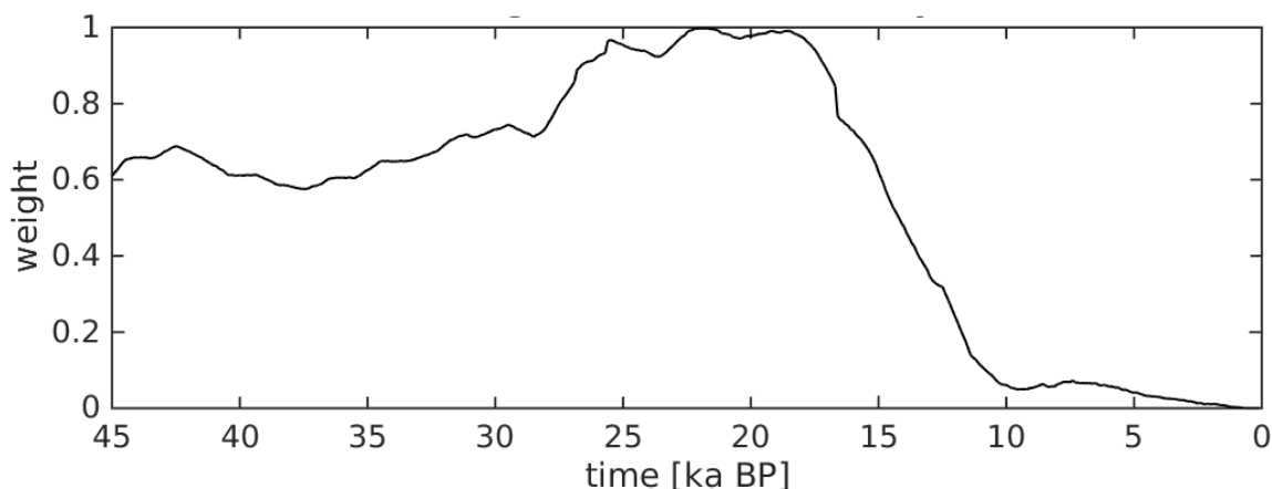
15 Figure A1: Transient weighting of MPI-ESM anomaly (LGM-PI). At LGM, the anomaly is fully described by MPI-ESM. CLIMBER2 anomaly weight is 1 - (\text{MPI-ESM anomaly}) .
