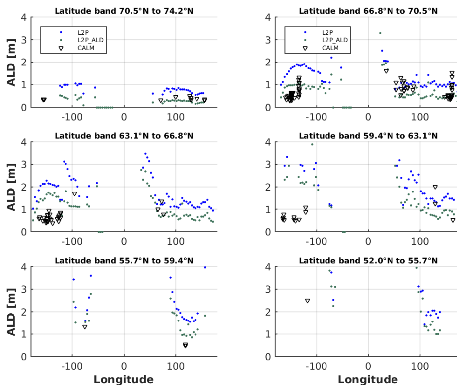
5 Figure A9: Latitudinal dependency of active layer depths inferred from JSBACH simulations (dots) and CALM observations (triangles). Blue dots represent the standard model experiment (L2P), green dots the sensitivity run with increased thermal insulation of the organic surface layer (L2P_ALD).
