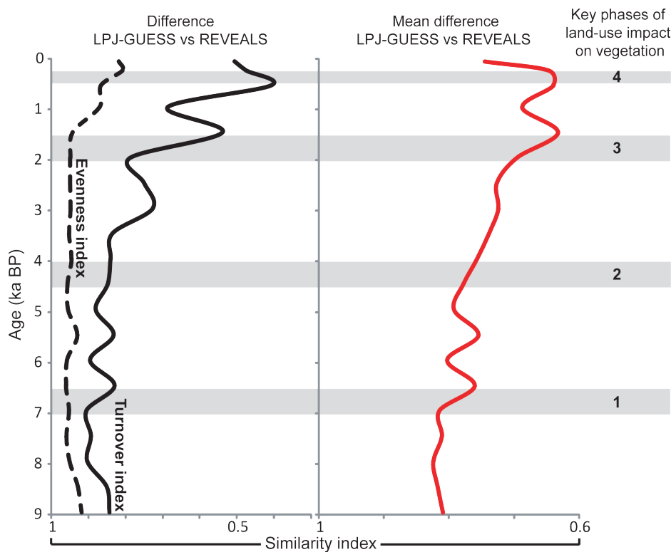
Figure 2: Differences between vegetation-change indices calculated based on LPJ-GUESS (dynamic vegetation model) simulations and pollen-based REVEALS estimates of past plant cover in Europe (Fig. 1). The differences are expressed by a similarity index ranging from 0 (no similarity) to 1 (total similarity). Left panel: similarity index for “evenness” and “turnover” indices. Right panel: mean of similarity indices for five vegetation-change indices. Marquer et al. (2017) assume that periods with low similarity indicate an impact of land use on vegetation. The four grey zones are major phases of land-use effects on land cover as identified by Marquer et al. (2017).
