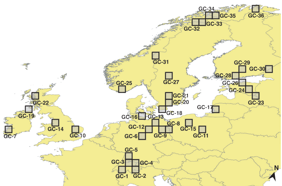
Figure 1: Location of the 36 1x1° grid cells used in Marquer et al. (2017) for Europe. Gridded pollen-based REVEALS estimates of plant abundance for the last 11.7 ka BP were calculated using all available pollen records in each grid cell.
