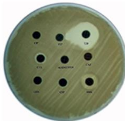
Figure 1. Modified double-disc synergy test (MDDST) showing synergy between cefepime (FEP)/ceftazidime (CAZ) and piperacillin-tazobactam (TZP)
