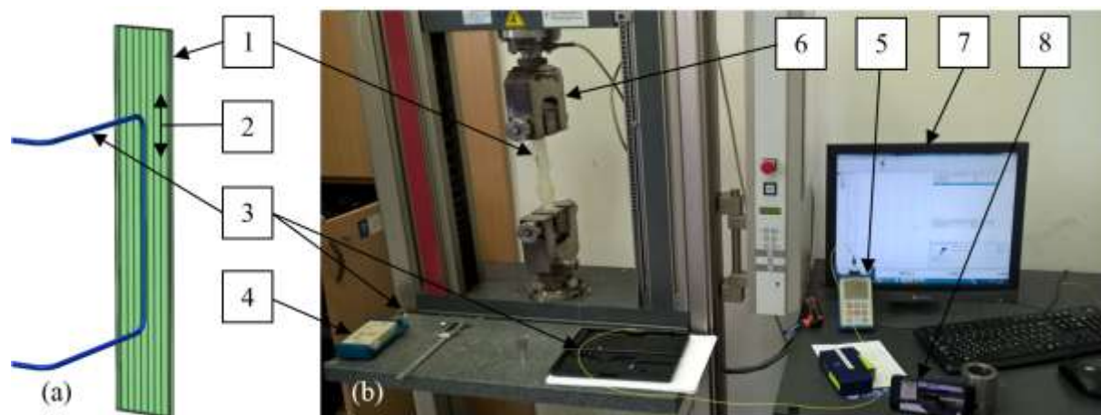
Figure 1. The specimen (a) and the measurement layout (b) (1–composite specimen, 2–direction of reinforcing fibre bundles, 3–optical fibre, 4–light source, 5–optical power meter, 6–clamps of the tensile tester, 7–values measured by the tensile tester, 8–video camera)
