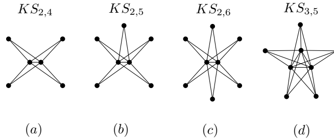
FIGURE 1. (a) The graph with 6 vertices with maximal irr. (b) The graph with 7 vertices with maximal irr. (c) and (d) Graphs with 8 vertices with maximal irr.
