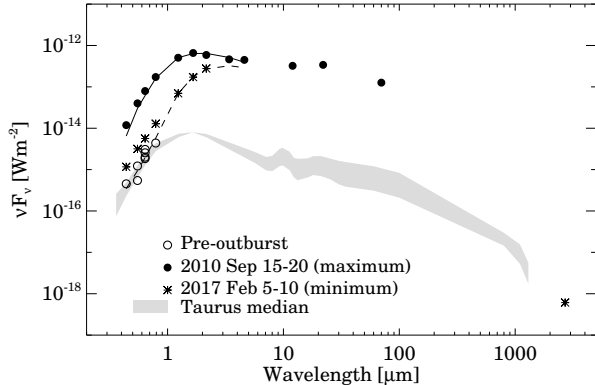
Figure 5. Optical-infrared-millimeter spectral energy distributions of V582 Aur at different phases of the eruption. Pre-outburst optical data are from Semkov et al. (2013). Data for 2010 September, representative of the maximum light of the outburst (Fig. 6), and for 2017 February, the minimum of the present dip, are from this work. The optical and near-infrared data in 2010 are supplemented by WISE observations from 2010 March 8 and 2010 September 15 (Sect. 3.3), and by a Herschel PACS 70\ \mu\text{m} data point obtained on 2012 Aug 27 (Marton et al. 2017). The shaded area marks the Taurus median scaled to the distance of V582 Aur, and reddened by A_V=1.53 mag interstellar extinction (data below 1.25\ \mu\text{m} and above 34\ \mu\text{m} are from D’Alessio et al. (1999), otherwise from Furlan et al. (2006)).
