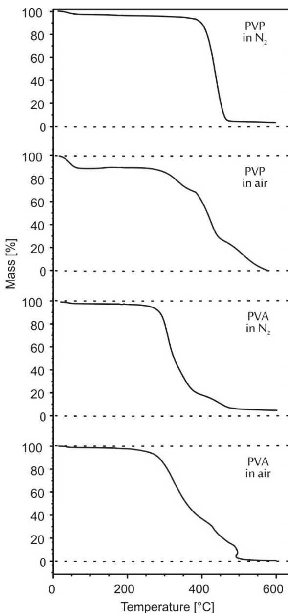
Fig. 3 – TG curves of the PVP and PVA nanofibers in N 2 and air.
