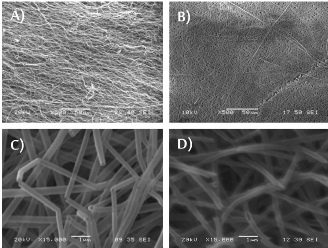
Fig. 2 – SEM images of A) PVA nanofibers B) Al 2 O 3 coated PVA nanofibers C) Al 2 O 3 nanotubes prepared by annealing from PVA/Al 2 O 3 nanocomposite D) Al 2 O 3 nanotubes prepared by dissolution from PVA/Al 2 O 3 nanocomposite.
