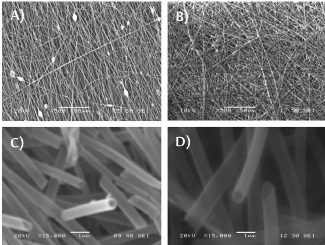
Fig. 1 – SEM images of A) PVP nanofibers B) Al 2 O 3 coated PVP nanofibers C) Al 2 O 3 nanotubes prepared by annealing from PVP/Al 2 O 3 nanocomposite D) Al 2 O 3 nanotubes prepared by dissolution from PVP/Al 2 O 3 nanocomposite.
