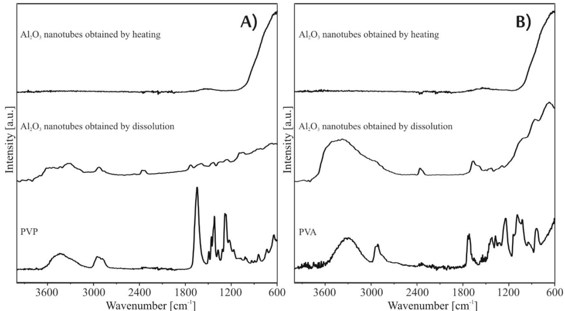
Fig. 4 – FT-IR spectra of the prepared samples, A) PVP nanofibers, Al 2 O 3 nanotubes obtained by dissolution from PVP/Al 2 O 3 nanocomposite, Al 2 O 3 nanotubes obtained by heating from PVP/Al 2 O 3 nanocomposite; B) PVA nanofibers, Al 2 O 3 nanotubes obtained by dissolution from PVA/Al 2 O 3 nanocomposite, Al 2 O 3 nanotubes obtained by heating from PVA/Al 2 O 3 nanocomposite.
