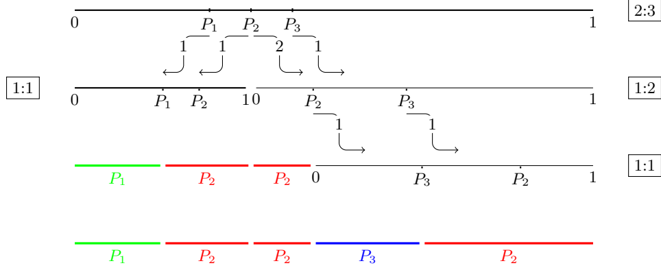
Fig. 1. The steps performed by our algorithm on Example 2. The colored intervals are the pieces already allocated to a player.
