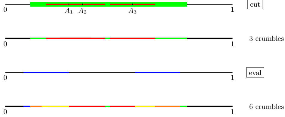
Fig. 2. The crumble partition after two queries in Example 5. We marked each of the 6 crumbles by a different color in the bottom picture.
