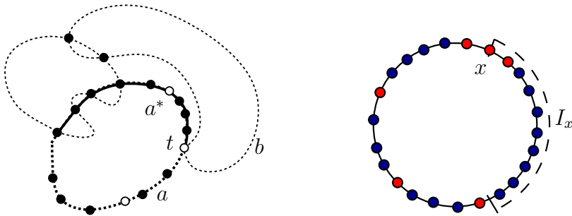
Figure 1: Left – The touching t is happy. The hollow points belong to T \cap a . The arc a^* \subset a satisfies |X \cap a^*| \geq \alpha_1 |T \cap a^*| with \alpha_1 = 5 . Right – Lemma 1. Each red point x \in R is contained in an arc I_x that satisfies w(B \cap I_x) \geq \lambda |R \cap I_x| . (In the depicted scenario w(x) = 1 for all x and we have \lambda = 4 .)
