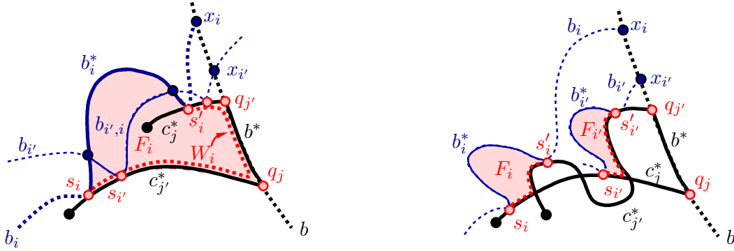
Figure 6: Proof of Claim 6. Left: If c_j^* and c_{j'}^* are disjoint, then any pair of curves b_i, b_{i'} with i, i' \in I_{q_j} \cap I_{q_{j'}} yields a lens b_{i',i} or b_{i,i'} . Right: If the arcs c_j^* and c_{j'}^* have multiple intersections, then a pair of curves b_i and b_{i'} can determine non-overlapping pockets F_i and F_{i'} . Thus, b_i and b_{i'} do not necessary determine a lens within F_i or F_{i'} .
