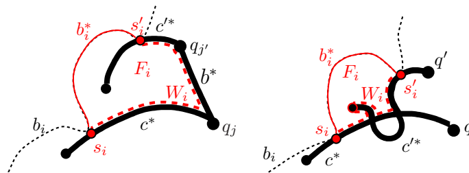
Figure 11: The portion W_i of W between s'_i = b_i \cap c' and s_i = b_i \cap c is traced. The face F_i of \mathbb{R}^2 \setminus (b_i \cup W_i) lies to the right of b_i . Left: The arcs c^* and c' are disjoint so both W and W_i must include b^* . Right: The scenario where c^* and c' intersect.
