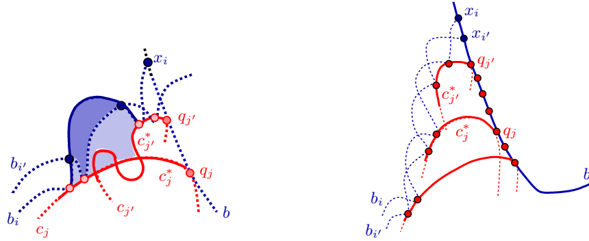
Figure 4: Left – In the first charging scenario, the poor touchings q_j, q_{j'} \in Q_i \cap Q_{i'} are close along b^* (so they can meet one another). As b_{i'} enters the pocket formed by the touchings between b_i and each of the curves c_j, c_{j'} , the curves b_i and b_{i'} define a lens of length l = O^*(k) which can send \Omega^*(1/k^2) units to q_j . Right – In the second charging scenario, the pairwise disjoint arcs c_j \in Q_i form the teeth of a comb-like arrangement.
