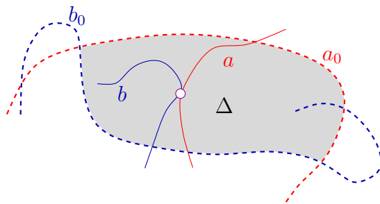
Figure 13: Proof of Lemma 6. We select a pair a_0, b_0 \in \mathcal{A} satisfying three properties including that at least |T|/(20h^2) of the touchings involve a pair of curves a, b \in \mathcal{A} \setminus \{a_0, b_0\} both intersecting a_0 \cup b_0 . We then choose an open cell \Delta \subset \mathbb{R}^2 \setminus (a_0 \cup b_0) which contains at least |T|/(2400fh^3) of these touchings.
