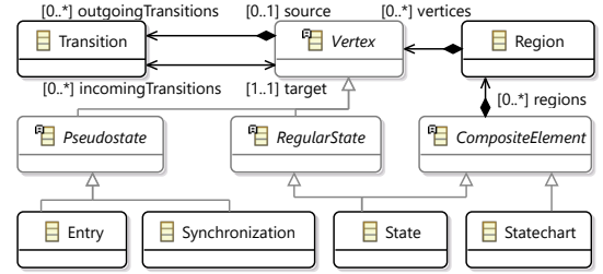
Figure 1: Metamodel of Yakindu statecharts
