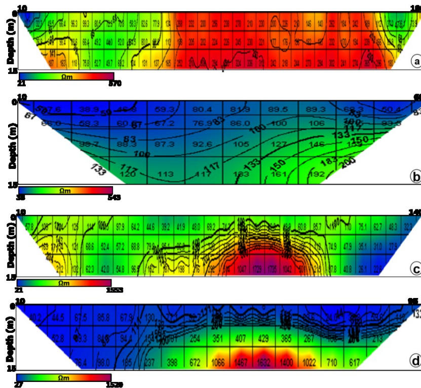
Figure 7: Resistivity Profiles or Pseudosections 1 to 4 at Location Two. Profiles 1 to 4 are taken along VES stations 5 to 8 in Figure 5.
