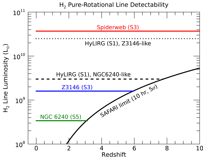
Figure 4. Detectability of H_2 pure-rotational lines for three known extreme H_2 emitters: (1) the Spiderweb radio galaxy at z = 2.16 with L(0-0 S(3)) = 3.7 \times 10^{10} L_{\odot} (Ogle et al. 2012); (2) Z3146 BCG at z = 0.29 with L(0-0 S(3)) = 1.6 \times 10^9 L_{\odot} (Egami et al. 2006a); (3) NGC 6240 at z = 0.0245 with L(0-0 S(3)) = 3.4 \times 10^8 L_{\odot} (Armus et al. 2006). The brightest line was used for each case. With SAFARI’s line sensitivity, which is also plotted (10 hours, 5\sigma ), the Spiderweb galaxy would be visible beyond z = 10 , while the Z3146 BCG would be visible up to z \sim 6 ; NGC 6240, on the other hand, would drop out at z \sim 3 . Also shown are the visibilities of a HyLIRG ( L_{IR} = 10^{13} L_{\odot} ) through the 0–0 S(1) line assuming L_{0-0 S(1)/ L_{IR} = 0.25\% (Z3146-like) and 0.03% (NGC 6240-like).
