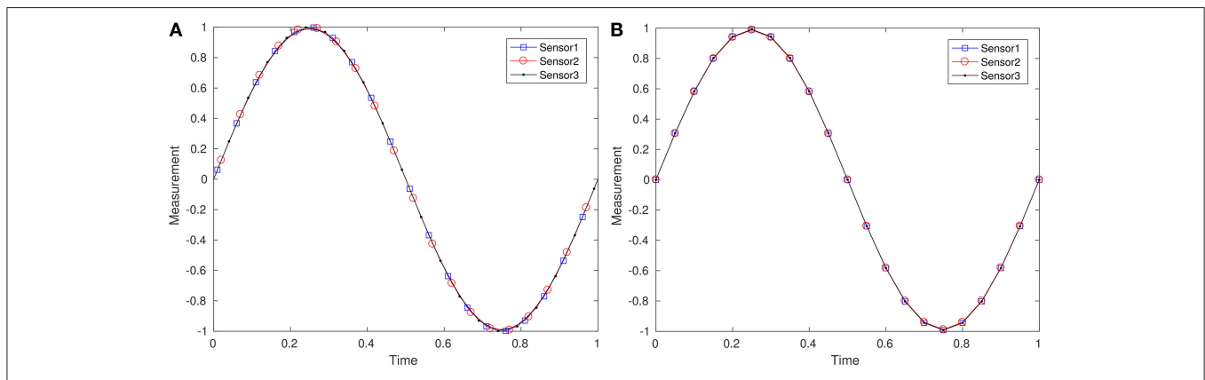
FIGURE 7 | Re-sampling on time-stamped data: (A) before re-sampling with irregular starting times, and (B) after re-sampling.
