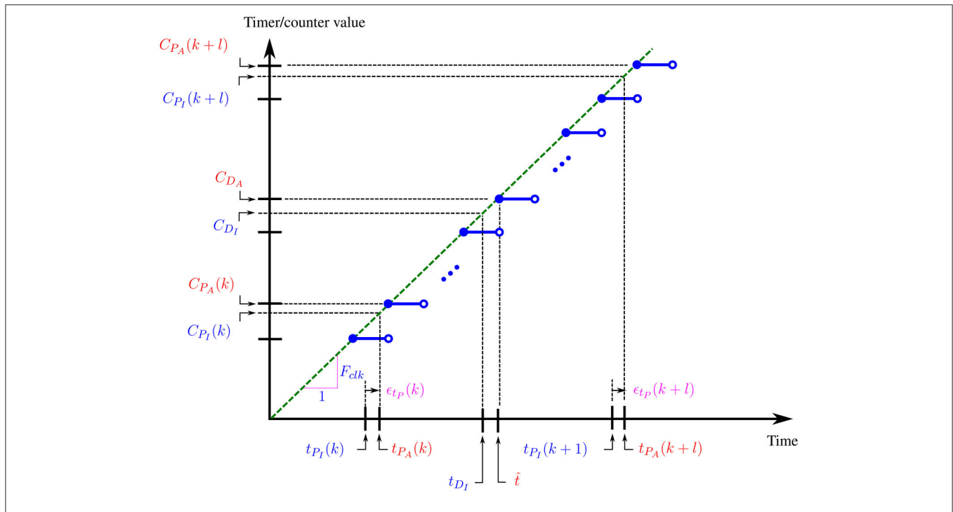
FIGURE 6 | Error analysis on proposed timestamping method.
