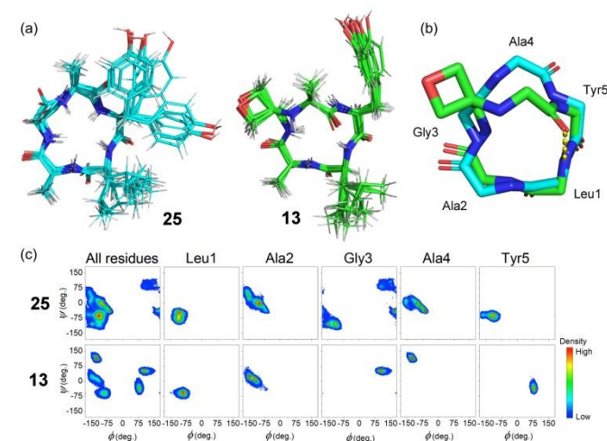
Figure 7 (a) NOE-restrained Molecular Dynamics simulations of cLAGAY ( 25 in cyan) and oxetane modified cLAGOXAY ( 13 in green). For each, a total of 10 representative structures are overlaid. (b) Peptide backbones of 13 and 25 with side-chains omitted for clarity. For 13 , intramolecular H-bond is indicated (yellow dots). (c) Ramachandran plots showing dihedral angles \psi against \phi for the amino acid residues within 13 and 25 .
