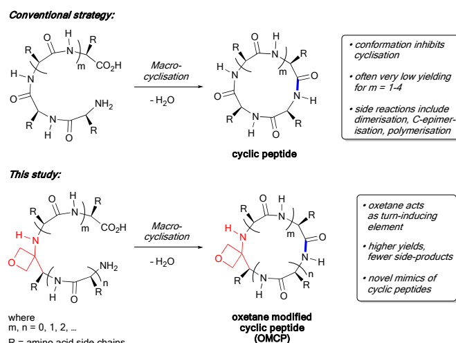
Scheme 1 Difficulties associated with making small cyclic peptides and improvements arising from oxetane introduction.
