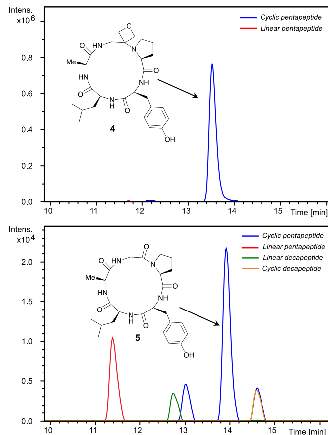
Figure 1 Extracted ion chromatograms of peptide macrocyclisations [DEPBT (2 equiv), i\text{Pr}_2\text{EtN} (2 equiv), DMF (0.001 M), 48 h, RT] for 1 → 4 (top) and 3 → 5 (bottom).
