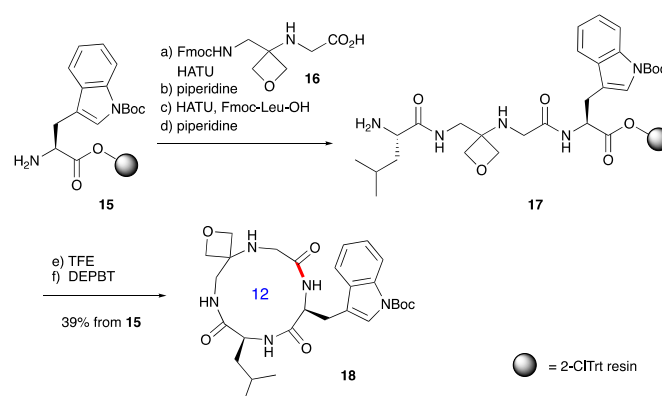
Scheme 4 Synthesis of oxetane modified cyclic peptide 18 by SPPS. Reaction conditions: (a) 16 (2 equiv), HATU (1.9 equiv), 1 Pr 2 EtN (4.0 equiv), DMF, 2–4 h, double coupling; (b) 20% piperidine, DMF, 20 min; (c) Fmoc-Leu-OH (5.0 equiv), HATU (4.9 equiv), 1 Pr 2 EtN (10 equiv), DMF, 1 h; (d) 20% piperidine, DMF, 20 min; (e) TFE/CH 2 Cl 2 (1:4), 3 × 1 h; (f) DEPBT (2.0 equiv), 1 Pr 2 EtN (2.0 equiv), DMF (0.001 M), 64 h.
