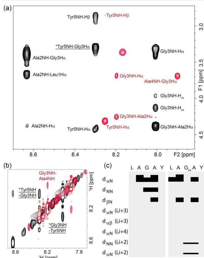
Figure 6 NOESY spectra of LAGOXAY-OMe (black) and LAGAY-OMe (red) collected with a mixing time of 400 ms for samples containing 30 mM peptide solubilised in d_6 -DMSO. Both spectra were collected at 298 K at a field strength of 700 MHz. Panel (a) shows the amide to \text{H}\alpha H \beta dipolar coupling in the fingerprint region, and panel (b) shows the sequential and medium-range amide proton coupling. Medium range NOEs are indicated by an asterisk and underlined. (c) NOE-connectivity maps of LAGOXAY-OMe and LAGAY-OMe based on NOE spectra collected with 250-800 ms mixing times. Each sequential and medium-range coupling is indicated on the left, and a bar is used to join the coupled residues if a coupling is observed.
