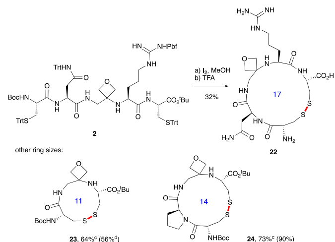
Scheme 5 Oxetane modified cyclic peptides by disulphide bond formation. Reagents and conditions: (a) I 2 (3.0 equiv), MeOH, 1 h; (b) 70% TFA / 20% CH 2 Cl 2 / 10% TIS, 2.5 h. b Bond formed in macrocyclisation indicated in red. c TFA step omitted; yield in parenthesis for the cyclisation of linear peptide with C=O rather than oxetane in backbone. d Data taken from ref 14.
