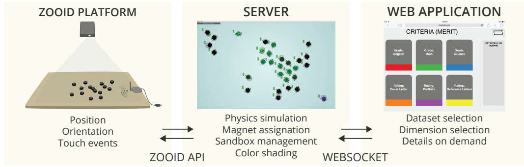
Fig. 9. Our implementation extends the original Zoids implementation [54] by adding connectivity to a web server with a generic client architecture. It makes it easy to develop new web applications to interact with Zoids.
