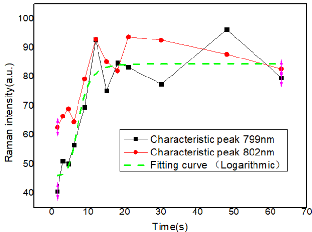
Fig. 8. Raman characteristic peak intensity of siphon process
