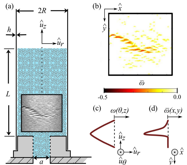
FIG. 2. (Color online) (a) Schematic cross-section of the experimental setup indicating its dimensions. L indicates the height of the granular column. A typical image used in our analysis is shown, marking the area of the shell it captures. Due to oblique illumination from above, the upper (lower) parts of diamond shaped indentations produce dark (bright) features in the image. (b) Field \bar{\omega} obtained from processing the image of the deformation pattern shown in (a). (c) Schematic representation of \omega(\theta, z) , for fixed \theta , of the cross-section at the center of a single diamond shaped indentation in the Yoshimura pattern. Referential directions corresponding to cylindrical coordinates (r, \theta, z) on the shell are indicated. Here \theta = \theta(x, y) and z = z(x, y) , with (x, y) Cartesian coordinates on the image, as indicated in (d). (d) Schematic representation of \bar{\omega}(x, y) , corresponding to the cross-section of the indentation shown in (c).
