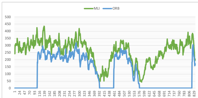
Fig. 9: The number of trusty inlier keypoints after graph optimization of ORB-SLAM which is a critical indicator displaying the tracking quality. MLI generates significantly better results than standard ORB under the dynamic light changing environment.
