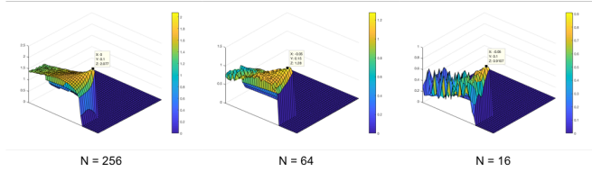
Fig. 5: Lowering the number of histogram bins (which is classical for image alignment tasks) leads to a difficult-to-optimize cost function landscape during illumination estimation process (axis represent parameters a and b of contrast band \mathbf{u} = (a, b)^\top ).
