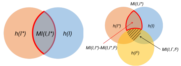
Fig. 3: Mutual information between two images (left), and three images (right) defined as the shared entropy between images.
