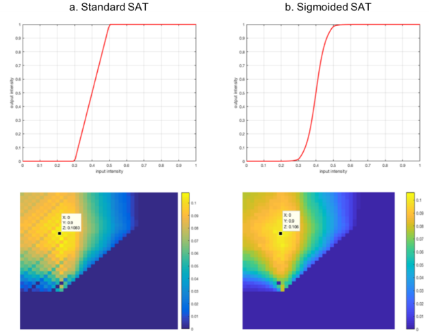
Fig. 6: Comparison between standard SAT function and sigmoid-smoothed SAT function wrt \mathbf{u} = (0.3, 0.5)^\top . Second row shows the conditional mutual information MI(I^*, I|I^0) computed by Eq. (8), notations keep as aforesaid for I^* and I with I^0 generated by the optimal contrast band from MI(I^*, f_{SAT}(I, \mathbf{u})) . We see clearly that standard SAT causes aliasing-like effect in the landscape, due to derivative discontinuity at cutting points a, b
