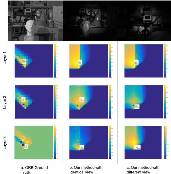
Fig. 7: In each layer, similar behaviors are shown with regard to optimums (see image a,b), compared with ORB detector. Ground truth for layers 2 and 3 are generated by a subtraction between the common keypoints detected from the previous optimal contrast band \mathbf{u}^* and the keypoints from all others contrast bands i.e. the ground truth of layer 2 is computed by removing all keypoints common with keypoints detected in previous optimum \mathbf{u}^* = (0, 0.15)^\top in layer 1. Empirical results also show that even with relatively different reference images (c), the landscapes are similar.
