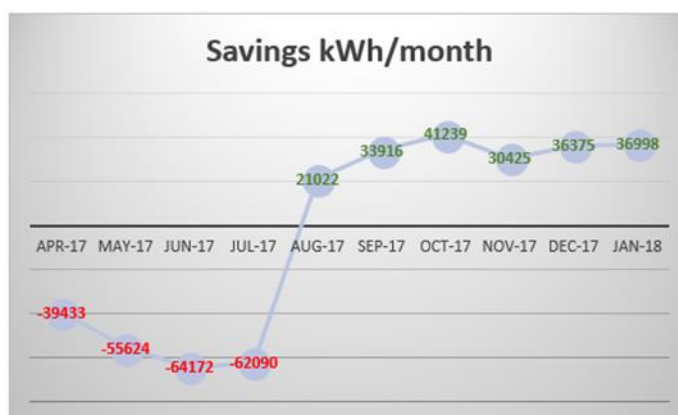
Figure 4 Electricity Consumption Data & Electricity Savings
