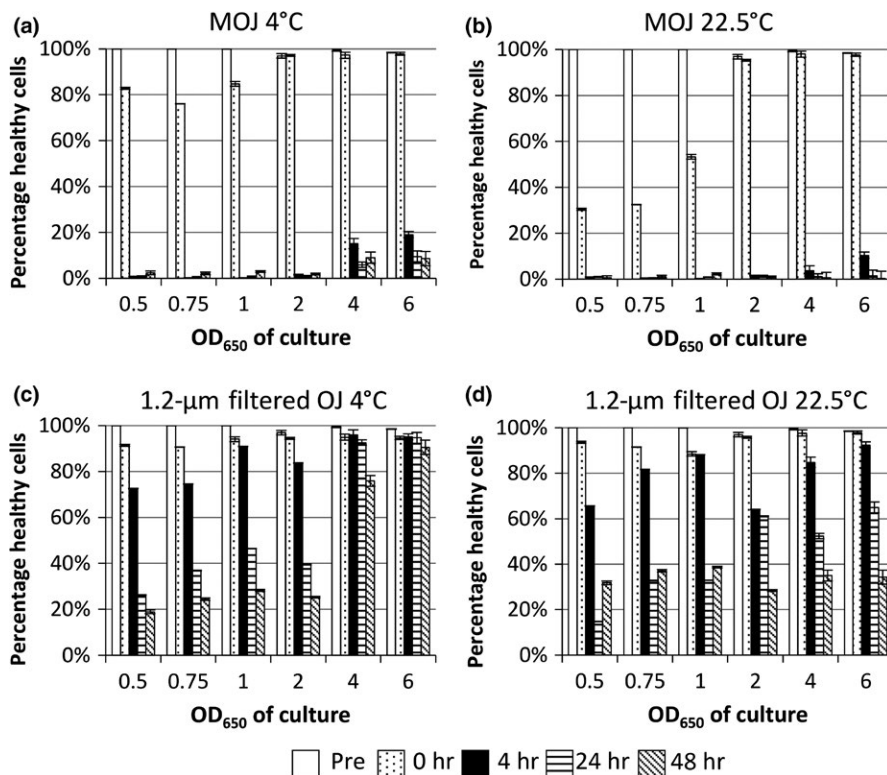
FIGURE 2 The effects of cell growth phase and incubation temperature on the viability of E. coli in 1.2-µm filtered orange juice (OJ) and model orange juice (MOJ). Cell viability and physiology were determined by FCM before addition to OJ or MOJ (Pre), immediately after addition (0 hr), and after 4, 24, and 48 hr. Mean percentage healthy cells ( PI^- BOX^- ) ± SD are shown for two independent cultures
