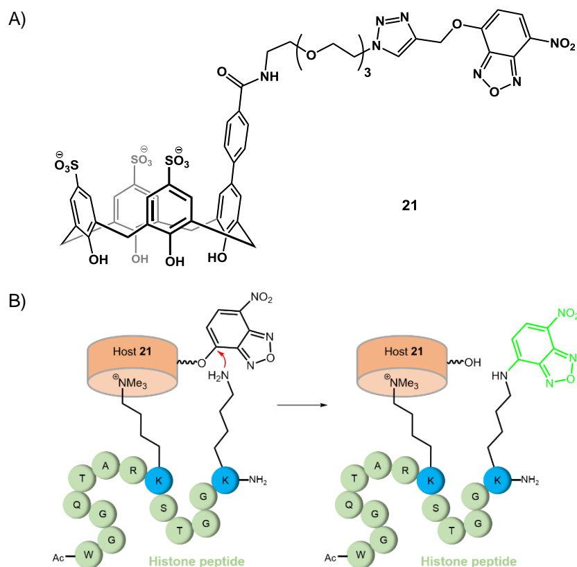
Scheme 8. A) Structure of NBD-labelled host 21 . B) After the selective binding of 21 to a trimethylated site of the peptide, a free lysine residue nearby reacts with the NBD moiety in an \text{S}_{\text{N}}\text{Ar} reaction.
