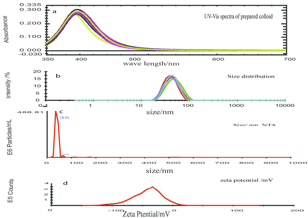
Characterisation of prepared nanoparticles, UV-Visible spectra, size distribution, size determination using NTA, and zeta potential as indicated in captions
