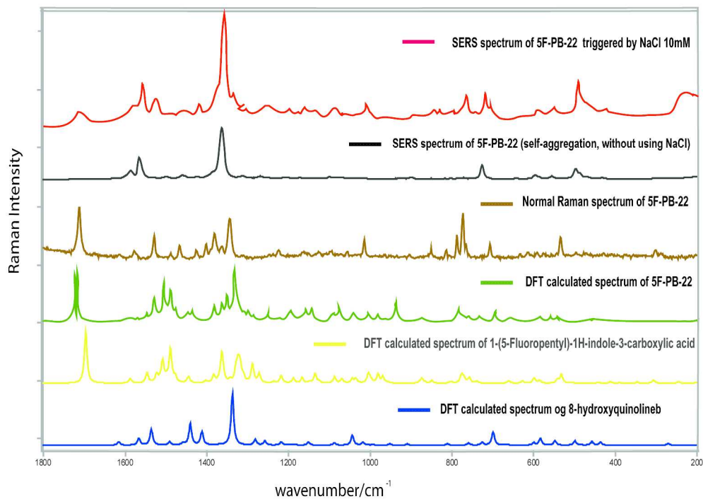
Experimental and DFT- calculated Raman spectra of 5F-PB-22, and its dissociation products as indicated in legend above each of spectra
