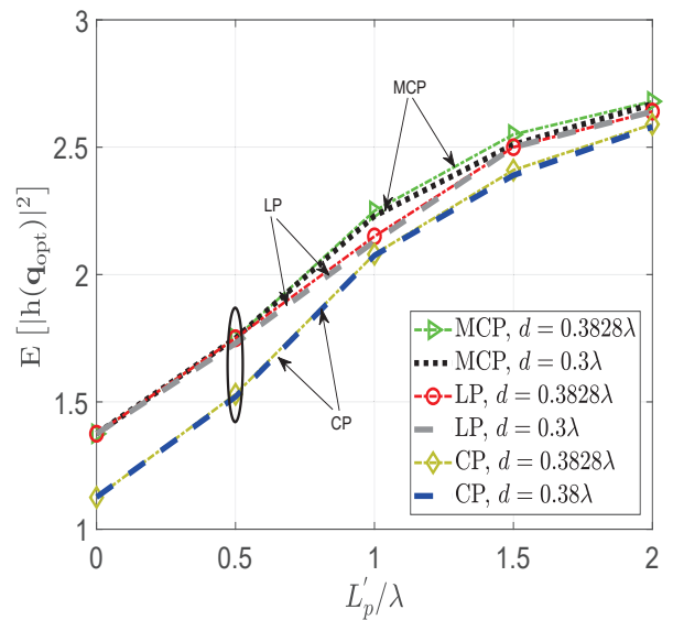
Fig. 3. \mathbb{E}[|h(\mathbf{q}_{opt})|^2] for different continuous paths, lengths and values of d with SNR = 10\text{dB} and \Delta = 0.05\lambda .
