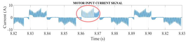
Figure 1: Motor current signal showing instability #4 at the centre.
