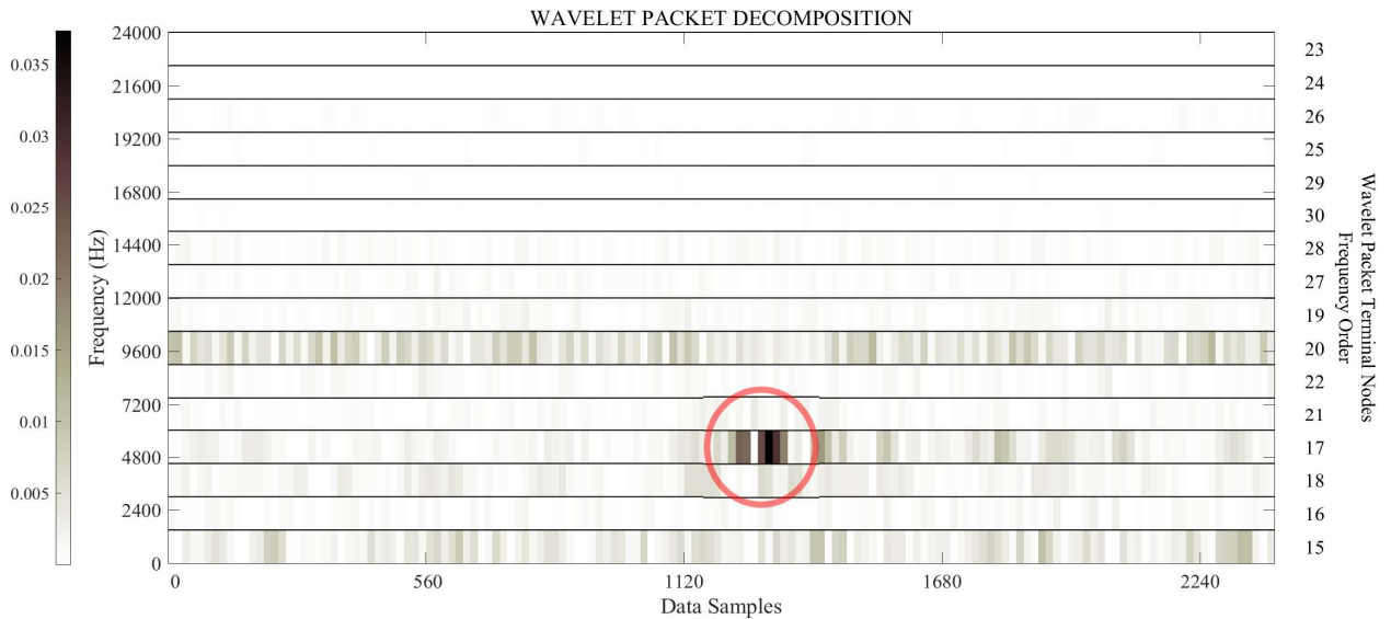
Figure 4: WPT dmev level 4 frequency ordered terminal node coefficients clearly showing the instability information in node 17.
