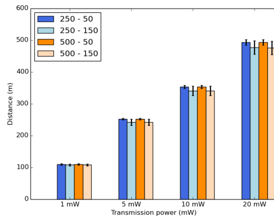
Figure 13. Average communication range.
