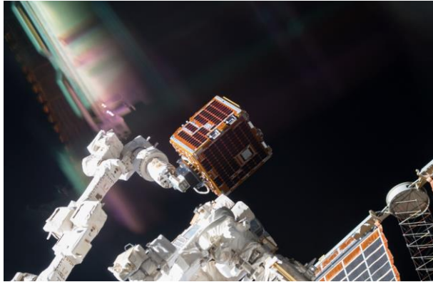
Figure 10. RemoveDebris mounted to the MSS SPDM ready for deployment
