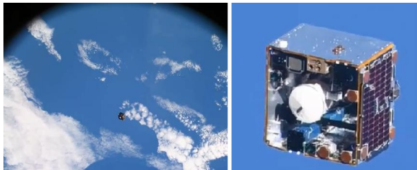
Figure 11. Left: RemoveDebris observed from the ISS shortly after deployment, Right: Close up of platform
