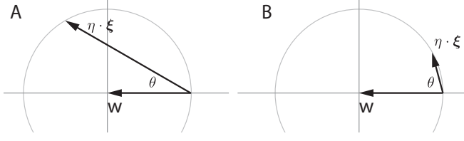
Figure 6. Alignment and learning rates. The larger \cos \theta , the larger the learning rate \eta that can be applied to unit vector \xi without w + \eta \cdot \xi leaving the unit circle.
