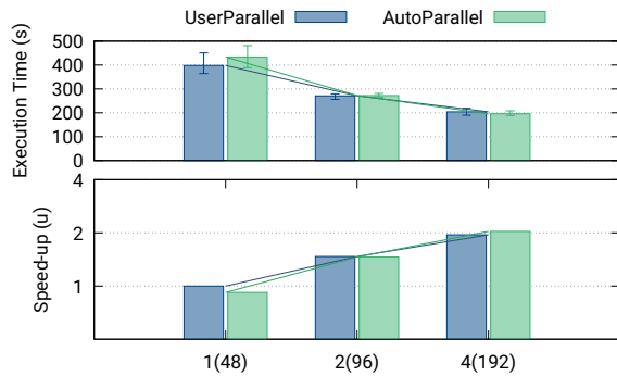
Figure 12. Cholesky decomposition: Execution times and speed-up
