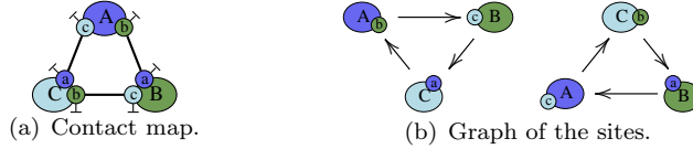
Fig. 10. ABC model. In 10(a), we recall the contact map. In Fig. 10(b), we give the graph of the sites that is associated with this contact map. The nodes of these graphs are the sites of the contact map. There is an oriented edge between a node s and a node t if and only if there is link in the contact map between the site s and a site of the protein that carries the site t but on a different site.
