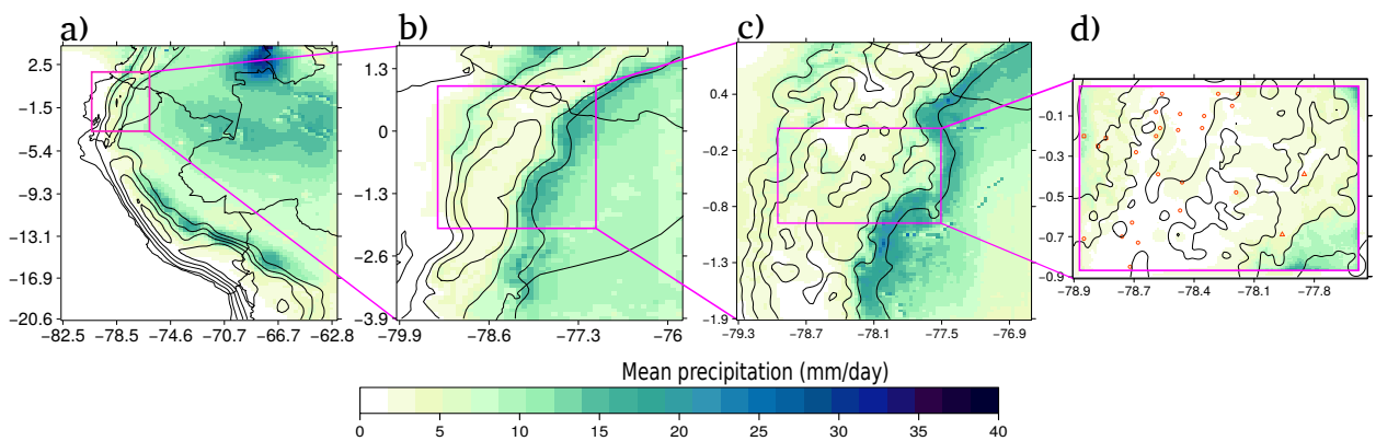
918 FIG. 2. Mean daily precipitation [mm day -1 ] during the 2014-2015 period of the four nested domains of the 919 WRF simulation a) WRF 27 km, b) WRF 9 km, c) WRF 3 km and d) WRF 1 km. Figure d) shows the exact 920 WRF domain, the WRF domain without the lateral boundary zone (purple box) and the stations (red dots). Note 921 that for station 12 and 18, we indicate the associated grid-point model used for the bias correction computations.
