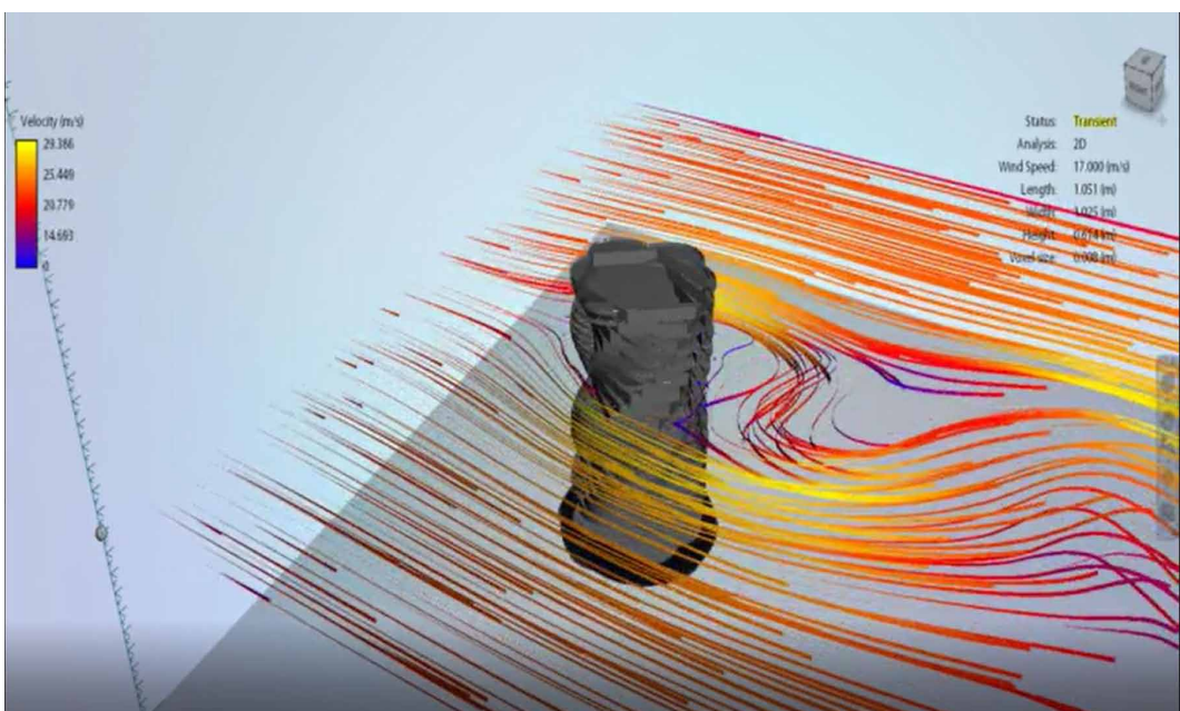
Figure 7. Workshop 3 wind analysis
