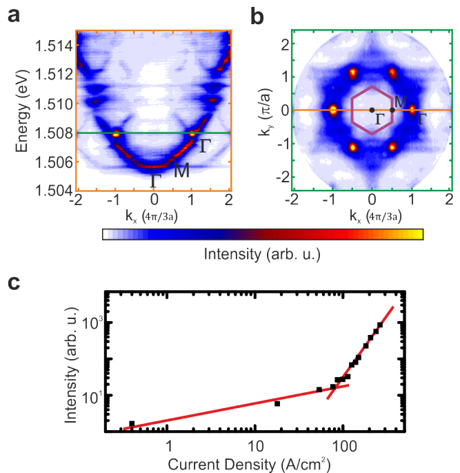
FIG. 3. (a) Luminescence dispersion of the honeycomb lattice in M- \Gamma -M direction under combined electrical and optical excitation. The constant laser power amounts to 90 Wcm -2 , while the injected current density amounts to 150 A/cm 2 here. With increasing current density a sharp emission in k-space as well as in energy is seen at the \Gamma -point of the 2nd Brillouin zone (BZ) at the bottom of the P-band. (b) Corresponding luminescence dispersion of the honeycomb lattice at a constant energy of 1.508 eV, as indicated by the green line in (a). The 1st BZ and the relevant high-symmetry points are highlighted. (c) Extracted intensity of the relevant mode under combined optical and electrical excitation. A nonlinear increase of the emission intensity is seen around a threshold density of \sim 100 A/cm 2 .
