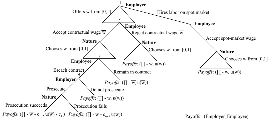
Figure 2: Game Tree.
