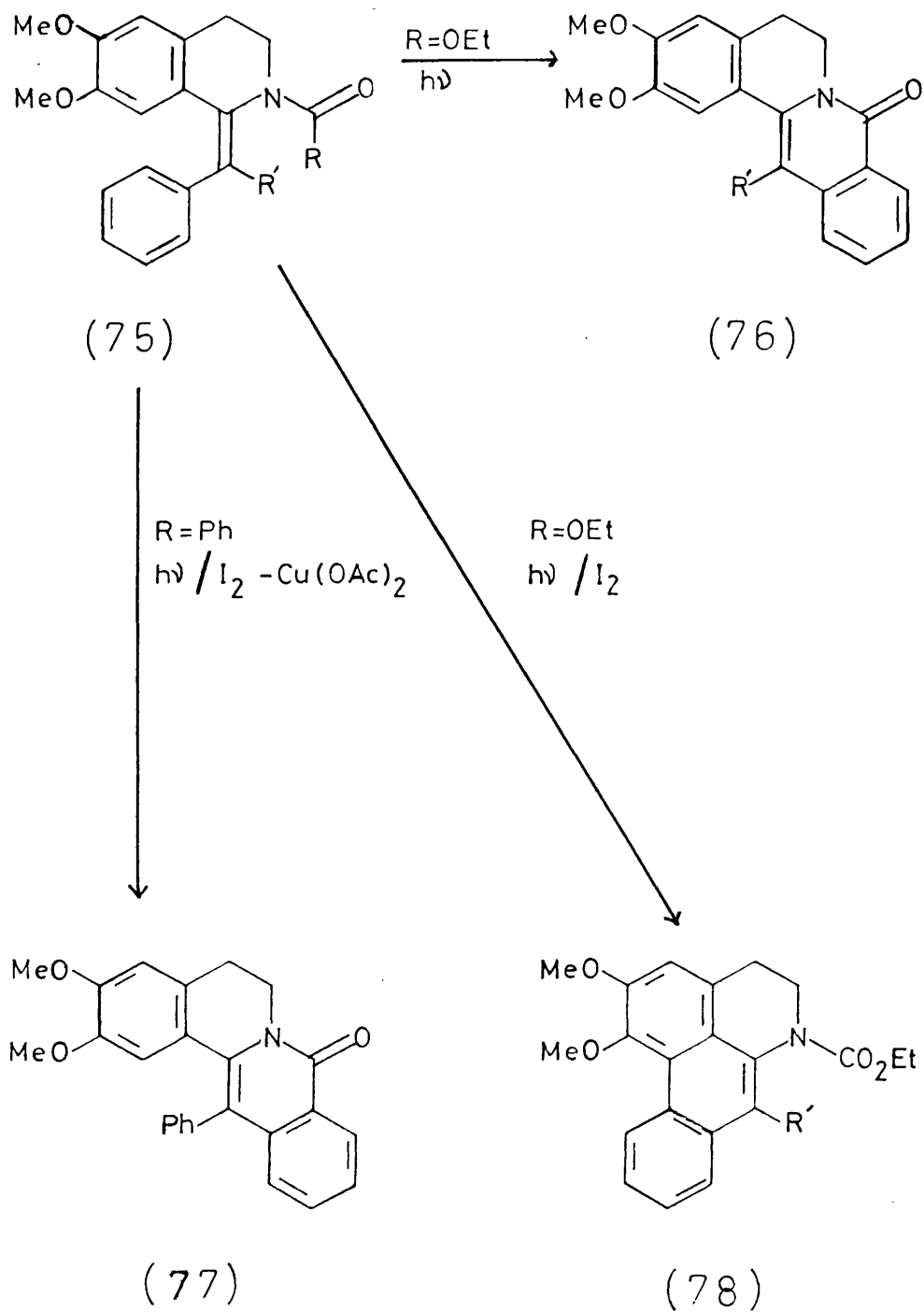
Scheme 20
