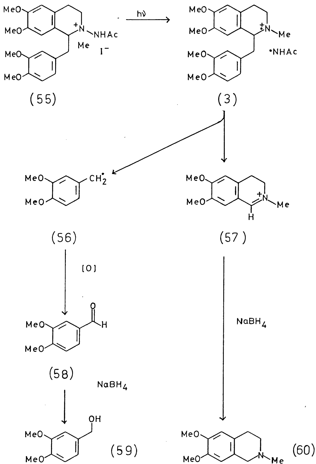
Scheme 18
