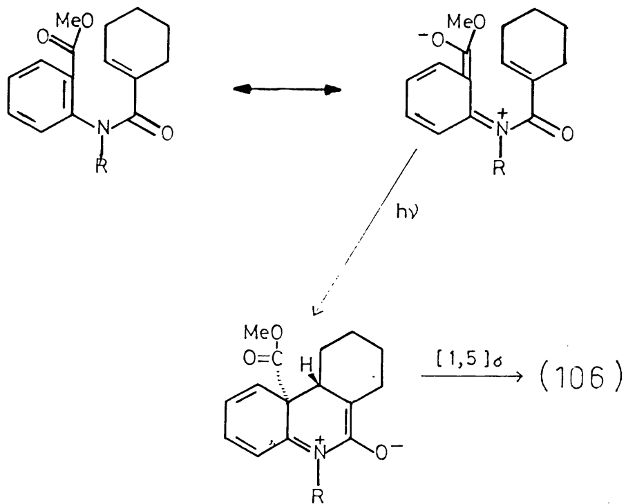
Scheme 27
