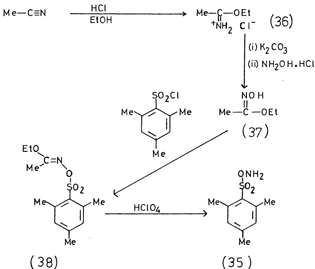
Scheme 15
