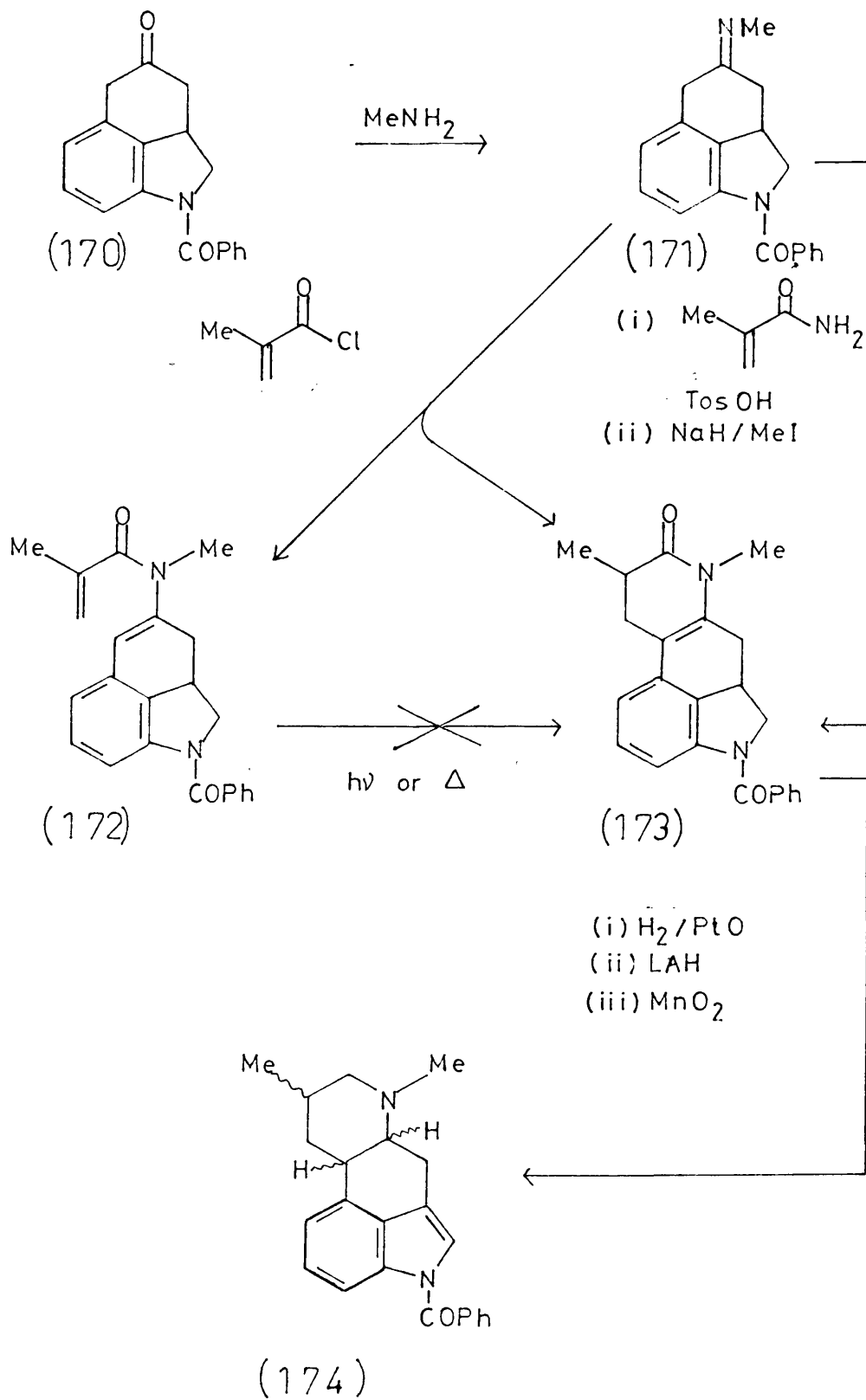
Scheme 39
