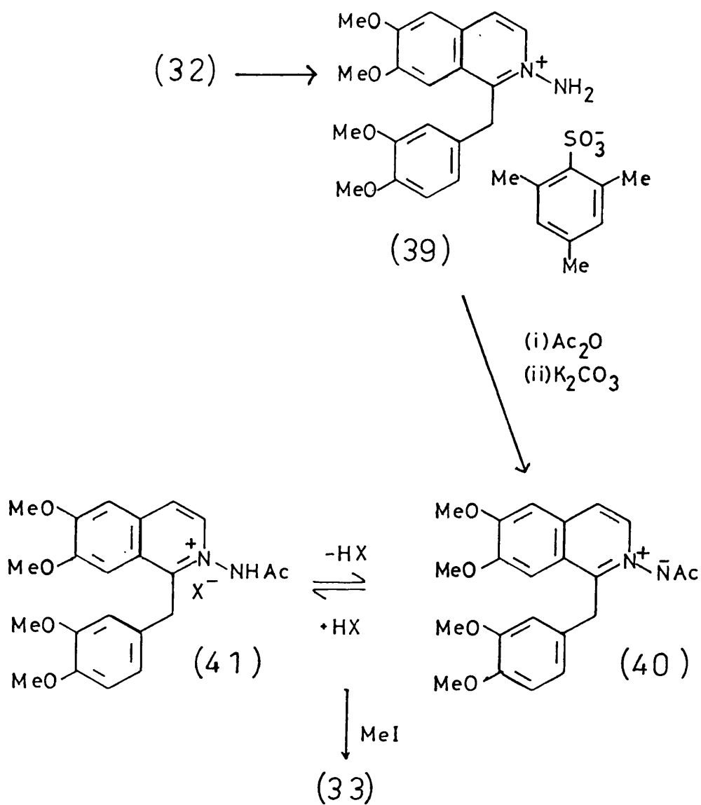
Scheme 16
