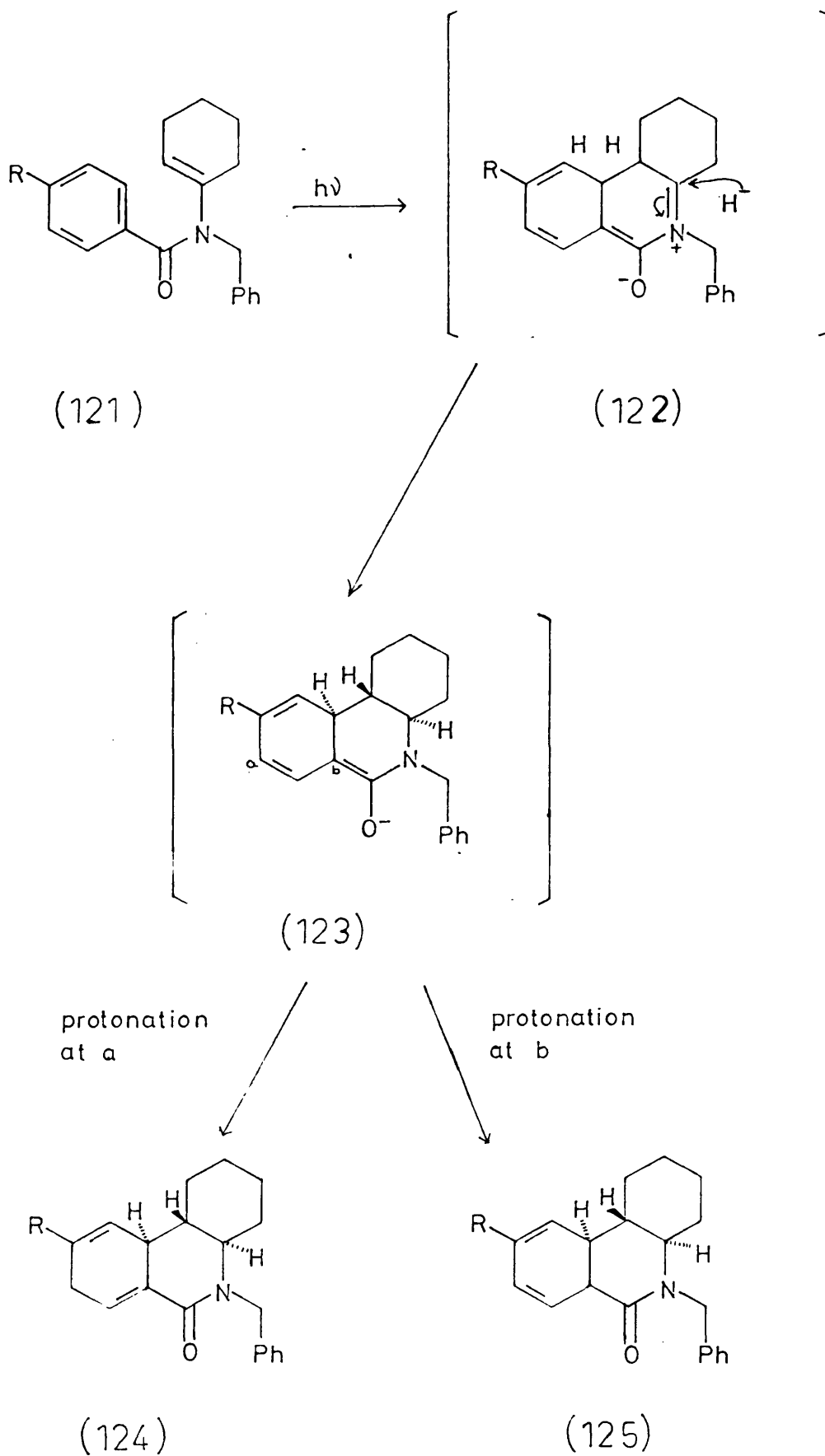
Scheme 29
