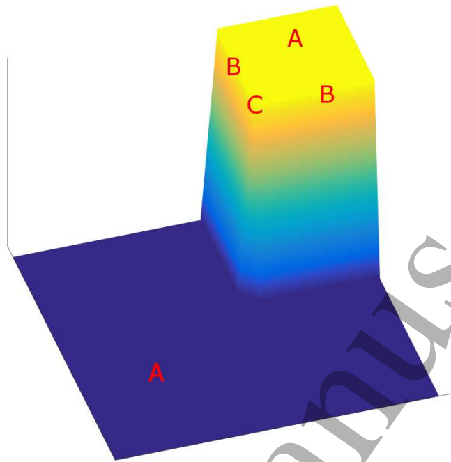
Figure 5: Surface representing a characteristic image, d , to demonstrate the behaviour of \Sigma and \Delta . Away from edges (A) we have \Sigma \approx \Delta \approx 0 . On simple edges (B) we have \Sigma \approx \Delta \gg 0 and, finally, at corners (C) we have \Sigma \gg \Delta .
