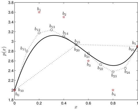
Fig. 2. Improvement in the range enclosure of p with a subdivision of an original interval \mathbf{x} . ( b_{10}, b_{11}, b_{12}, b_{13}, b_{14}, b_{15} ), and ( b_{20}, b_{21}, b_{22}, b_{23}, b_{24}, b_{25} ) are the Bernstein coefficients over \mathbf{x}_1 = [0, 0.5] and \mathbf{x}_2 = [0.5, 1] , respectively.
