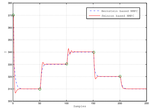
Fig. 3. Evolutions of the state C_A and T with NMPC based on Bernstein algorithm BBBC and MATLAB based fmincon function. Green circles at 0, 50, 100, 150, and 200 indicates the samples at which the set-point changes are implemented for T . The set-points are as follows: at 0 sec 310 K, at 50 sec 330 K, at 100 sec 340 K, at 150 s 320 K, and at 200 sec 310 K.
