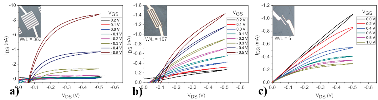
Figure 3: I-V Output characteristics of water-gated organic transistors based on pentacene (a), P3HT (b) and PEDOT:PSS (c). Inset of each panel shows the source-drain electrode geometry.
