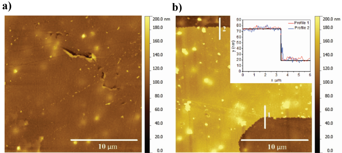
Figure 2: On the left, AFM image of a bare test pattern showing the morphology of the PEN substrate. On the right, an image of the source-drain electrode. Inset: electrode height profile.
