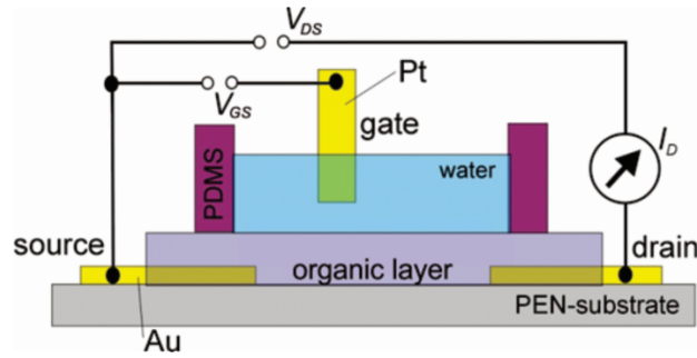
Figure 1: Schematic layout of the water-gated organic transistor. Source-drain electrodes are covered by the organic layer. A PDMS reservoir confines the aqueous solution onto the active layer.
