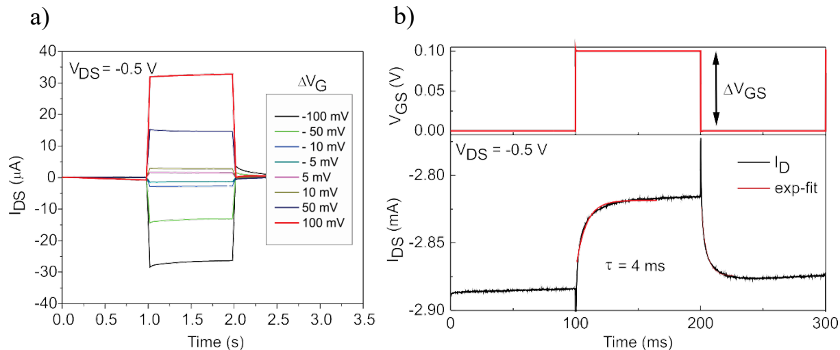
Figure 4: (a) Potentiometric sensing experiment showing high sensibility of I_{DS} to small gate potential variations ( \Delta V_G ) for a PEDOT:PSS OECT ( V_{DS} = -0.5 V ). (b) Operational speed plot for a PEDOT:PSS OECT showing estimated switching times approximately 4 ms ( V_{DS} = -0.5 V ).
