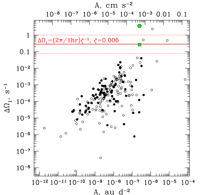
FIG. 1.— Change of the spin rate due to non-gravitational forces accumulated over a single orbit \Delta\Omega_1 (assuming lever arm parameter \zeta = 1 ), computed for a sample of 209 Solar System comets with available data on the amplitude of the non-gravitational acceleration. This parameter measures object's potential for rapid spin evolution; A is the normalization of a_{\text{ng}} at 1 au, assuming a_{\text{ng}}(r) profile from Marsden et al. (1973). Filled hexagons represent objects with measured sizes; empty ones have no size information available and we set radius R = 10 km for them. Green hexagon and square represent 'Oumuamua (we set A = A_1 for it) and correspond to \Delta\Omega_1 and \Delta\Omega_1^{(1-3)\text{au}} . Horizontal solid curve describes rotation rate change of 2\pi \text{ hr}^{-1} (i.e. spin-up to 1 hr period from a non-rotating state) for \zeta = 0.006 (corresponding to the mean of \log \zeta ); dashed lines illustrate 1\sigma deviation in \log \zeta , see equation (4). See text for more details.
