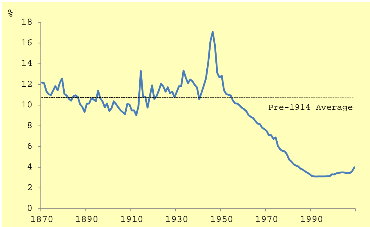
Figure 4: Narrow Money to Income Ratio
