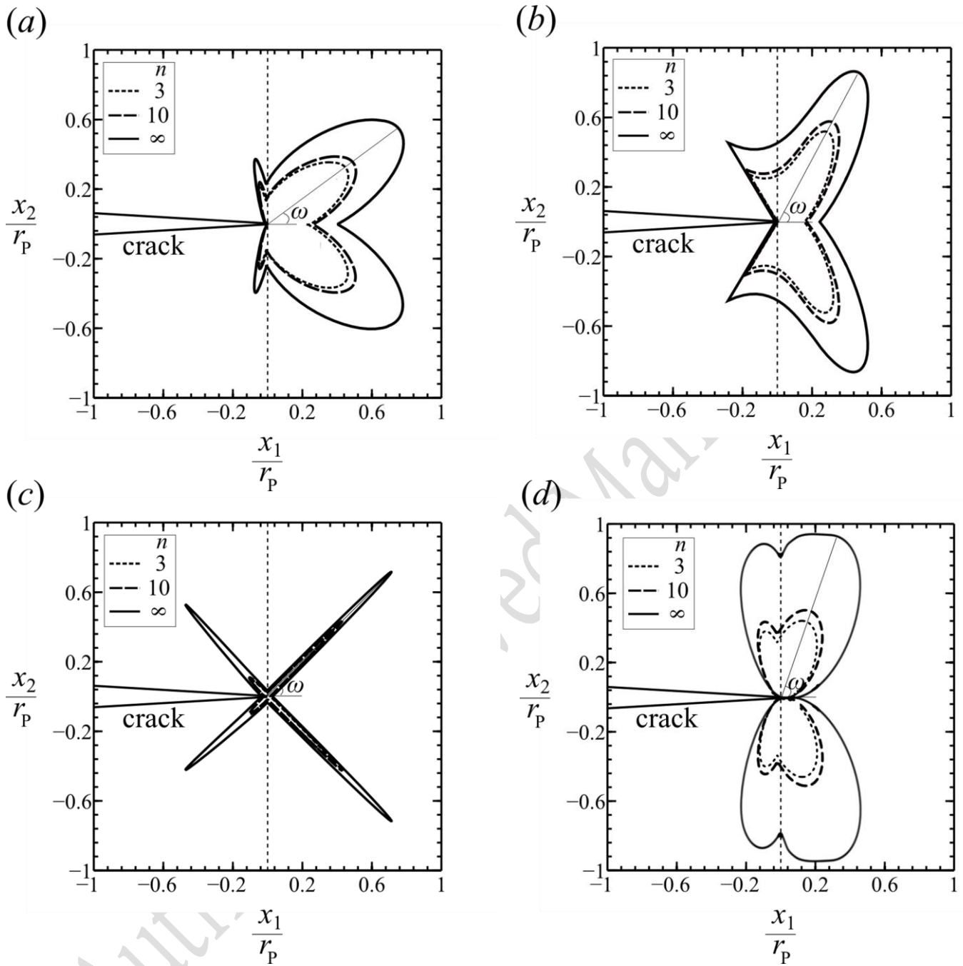
Fig 2. Mode I plastic zone for (a) triangular lattice, (b) kagome lattice, (c) diamond lattice, (d) hexagonal lattice.
