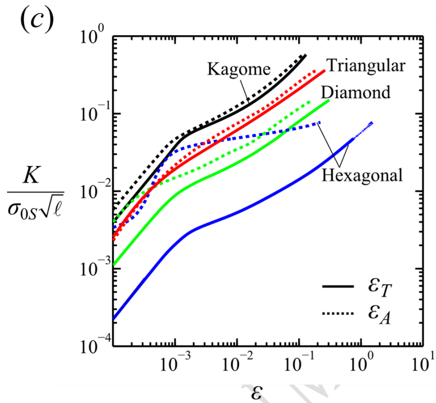
Fig 5. Mode I fracture toughness of the four topologies for \bar{\rho} = 0.05 and n = 10 according to (a) local tensile strain (LTS) criterion, (b) average tensile strain (ATS) criterion. (c) A comparison of predictions by the LTS and ATS criteria for the finite strain case.
