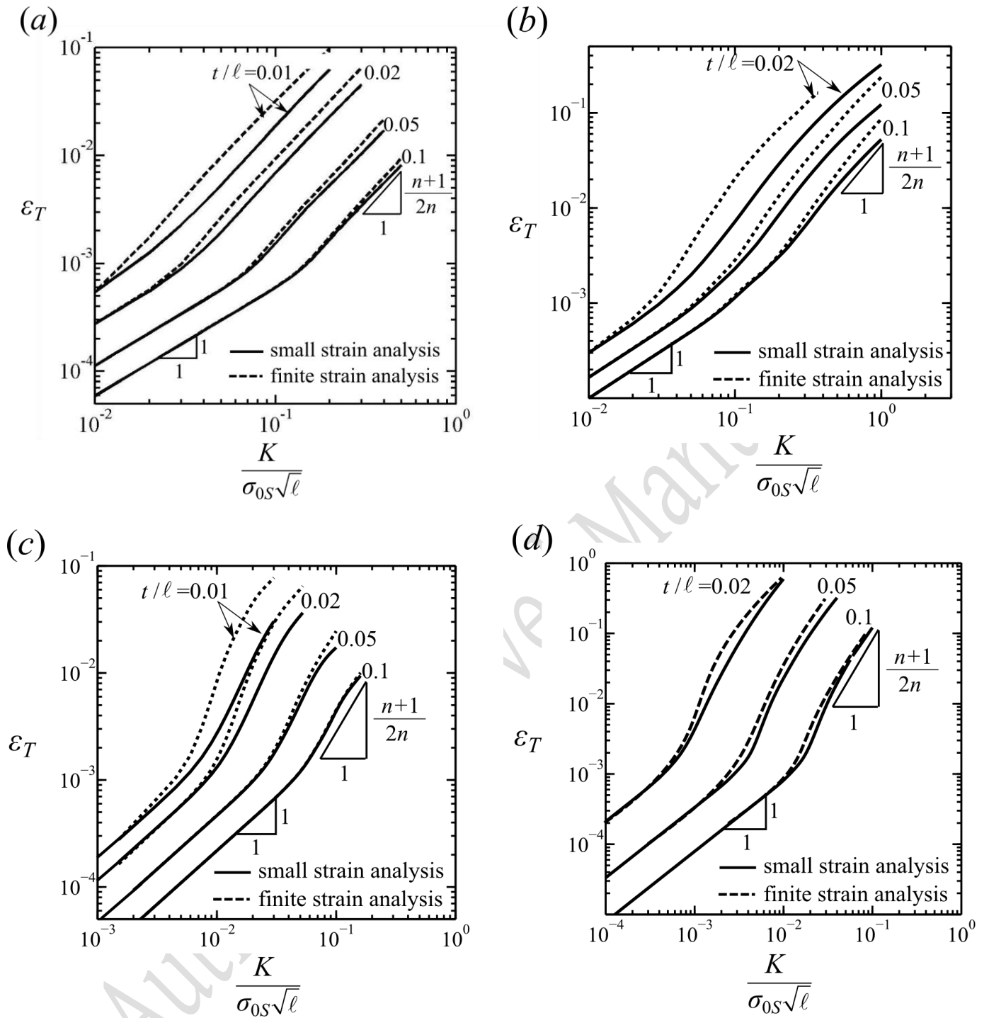
Fig 4. Maximum value of strain in the lattice cell wall for (a) triangular lattice, (b) kagome lattice, (c) diamond lattice, (d) hexagonal lattice.
