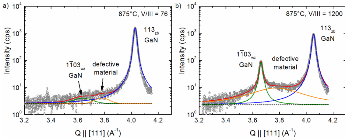
Figure 1 XRD intensity profile through the 1\bar{1}03_{wz} and 113_{zb} reflections (grey circles) for the samples grown on a 4^\circ miscut substrate at 875^\circ\text{C} and a V/III-ratio of (a) 76, and (b) 1200. Pseudo-Voigt fits for the zb-phase (blue), wz-phase (green), and defective zb-GaN material (orange) were used to estimate the phase fractions.
