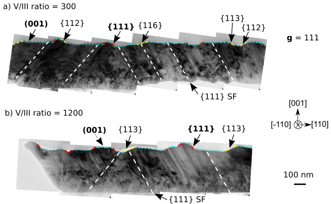
Figure 10 Bright-field TEM images of the samples grown at a temperature of 875 °C and (a) V/III-ratio of 300, (b) V/III-ratio of 1200. Imaging conditions: zone axis = [-110], g = 111 . For both (a) and (b), the typical {111} stacking fault orientations are indicated by the white dashed lines, the (001) surface by the blue dotted lines, {111} facets by the red dashed lines, and other facets by yellow dashed lines. The facets in (b), the {111} facets in particular, are larger and more pronounced than in (a).
