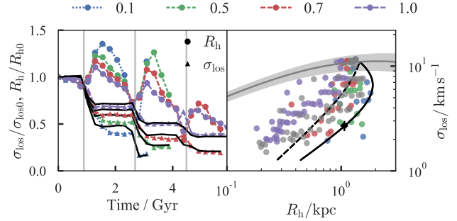
Figure 7. Observed properties of tidally-disrupted dSphs with varying equal inner stellar ( \gamma_\star ) and dark matter ( \gamma_{\text{DM}} ) density slope (blue \gamma = 0.1 , green \gamma = 0.5 , red \gamma = 0.7 and purple \gamma = 1 ). The left panel shows the evolution of the projected velocity dispersion (triangles) and half-light radius (circles). Overplotted in black are the predictions for the projected velocity dispersion from the central mass loss. Pericentric passages are shown by grey lines. The right panel is a version of the bottom panel of Fig. 2 with this set of models and the s = 1 spherical models of Section 3 shown in grey.
