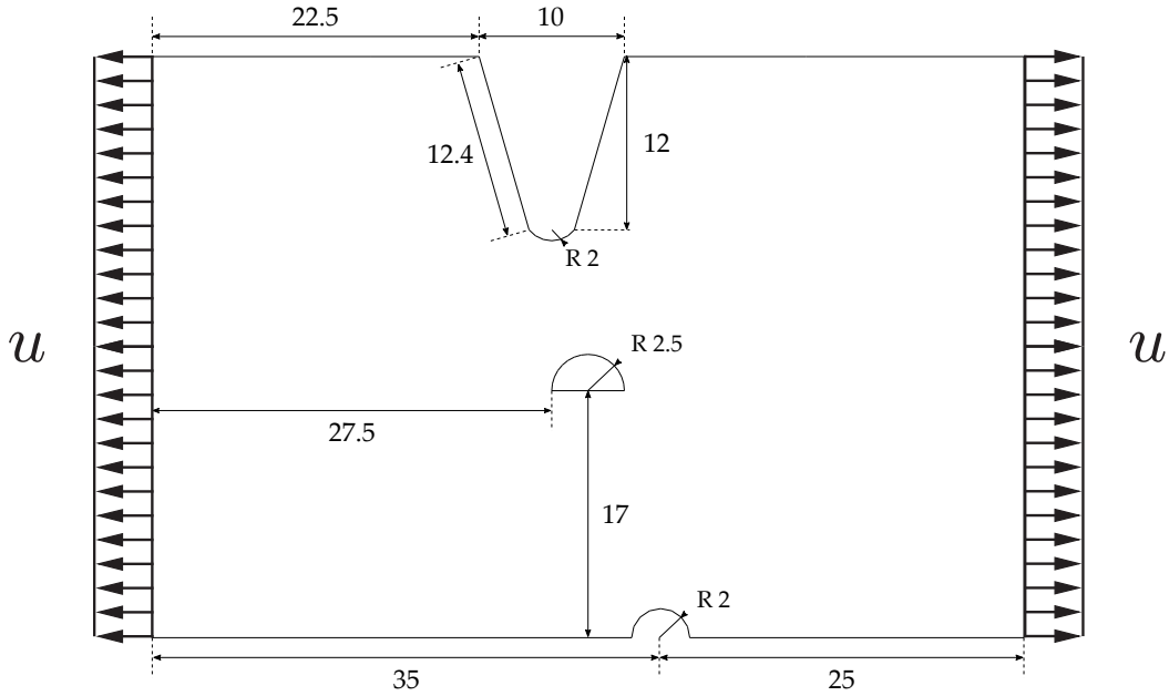
Figure 16: Geometry and loading configuration of a plate with existing defects, dimensions are given in mm. The defects are introduced in the initial rectangular geometry by prescribing the initial condition \phi = 1 .
