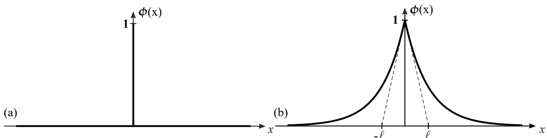
Figure 1: Sharp (a) and diffusive (b) crack topologies.
