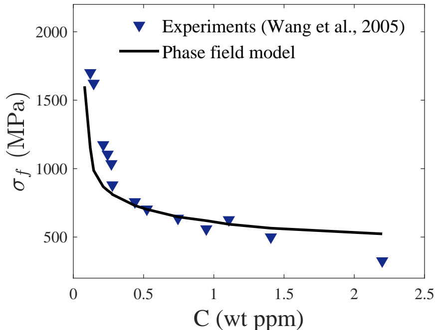
Figure 11: Notched bar subjected to tension test. Net section strength \sigma_f as a function of the hydrogen concentration C in AISI 4135 steel. Material properties: E = 210 GPa, \nu = 0.3 , \bar{V}_H = 2000 mm 3 /mol, D = 3.8 \times 10^{-5} mm 2 /s, \ell = 0.015 mm, and G_c = 64 KJ/m 2 .
