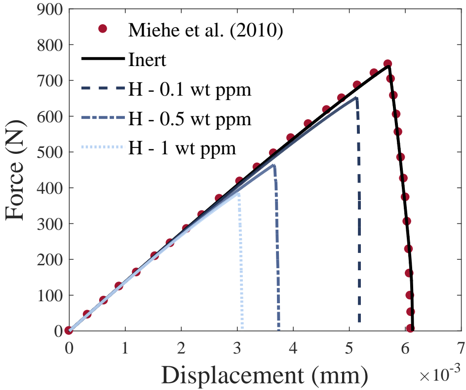
Figure 7: Cracked square plate subjected to tension. Load-deflection curves for different environments. The computations for C_0 = C_b = 0 wt ppm match the results by Mieke et al. [39] (symbols). Material properties: E = 210 GPa, \nu = 0.3 , G_c = 2.7 KJ/m 2 , \ell = 0.0075 mm, \bar{V}_H = 2000 mm 3 /mol, \ell_C \gg \ell , and T = 300 K.
