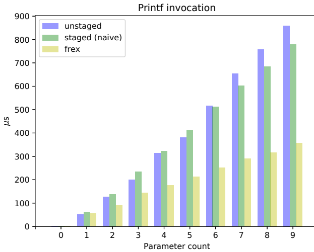
Fig. 28. Printf performance improvements
