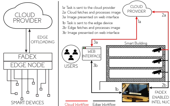
Figure 1: FADEX Architecture and Use Case
