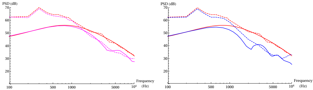
(a) Straight edge c = 0 red, and serrated edge c = 2 pink. (b) Straight edge c = 0 red, and serrated edge c = 4 blue.
