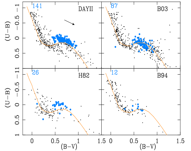
Figure 7. (U - B) , (B - V) diagram by DAYII, B03, H82 and B94. The orange line represents the ZAMS, shifted by values E(B - V)=0.22 , E(U - B)/E(B - V)=0.74 . An arrow shows the direction and length of the reddening vector in the upper left panel. Blue points denote the UF stars in common. Their respective numbers are quoted in each panel.
