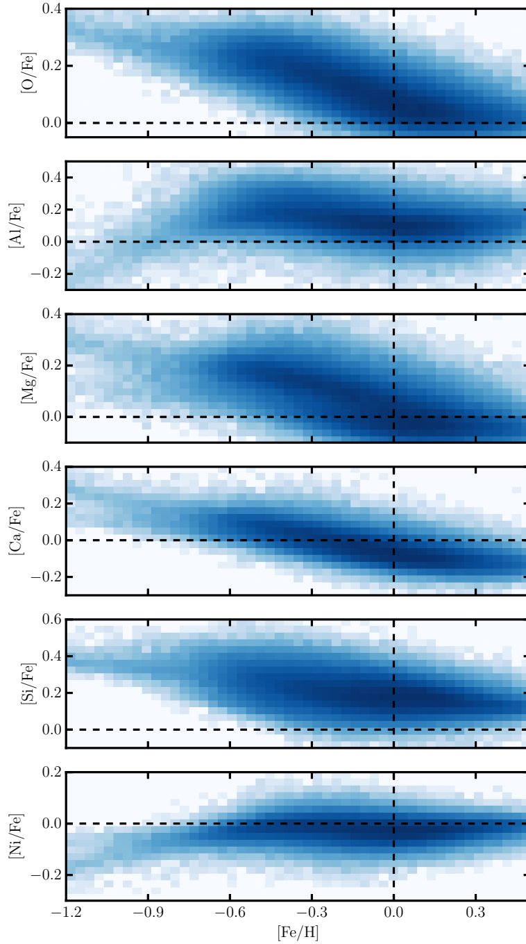
Fig. 17.— Detailed chemical abundances ( [X/Fe] ) for giant stars in RAVE-on with respect to [Fe/H] , showing the Galactic chemical evolution derived for each element. Bin densities are scaled logarithmically. Note that the y-axis limits vary for each panel, however for clarity we show the scaled-solar position by dashed lines, and have common tick mark spacing on the y-axis for all panels. Only stars meeting our quality constraints are shown (see Section 5).
