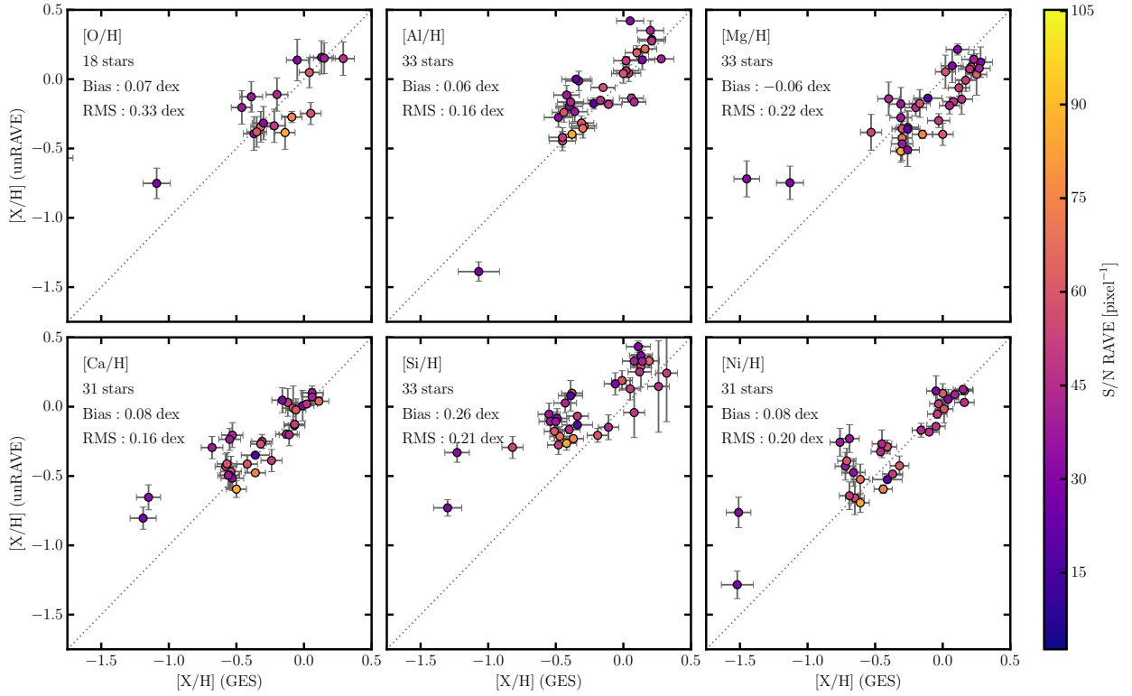
Fig. 13.— Detailed chemical abundances in the fourth internal data release from the Gaia-ESO survey compared to this work. The number of stars shown in each panel is indicated, and the bias and RMS deviations are shown. Stars are colored by the S/N of the RAVE spectra.
