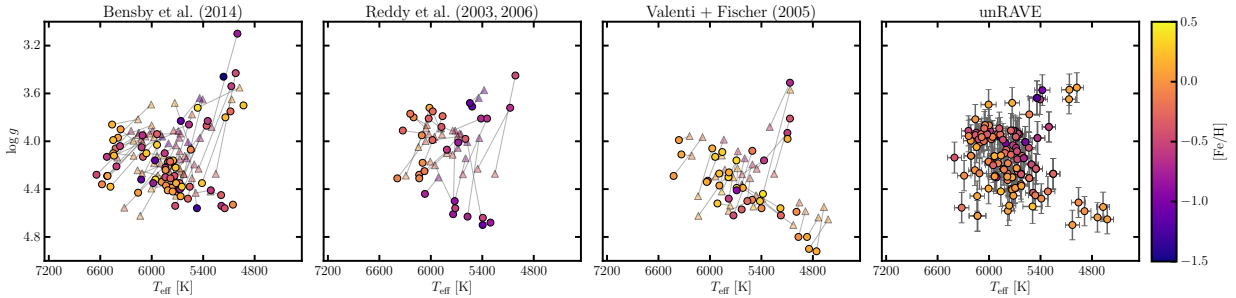
Fig. 10.— Hertzsprung-Russell diagrams of stars in common between this work and that of Bensby et al. (2014); Reddy et al. (2003, 2006); Valenti & Fischer (2005). Stars are colored by the metallicity of each study. Circles indicate literature markers in the first three panels, and the linked triangles indicate RAVE -on parameters for the same object. This figure illustrates the good qualitative agreement in the shape of the turnoff and sub-giant branch.
