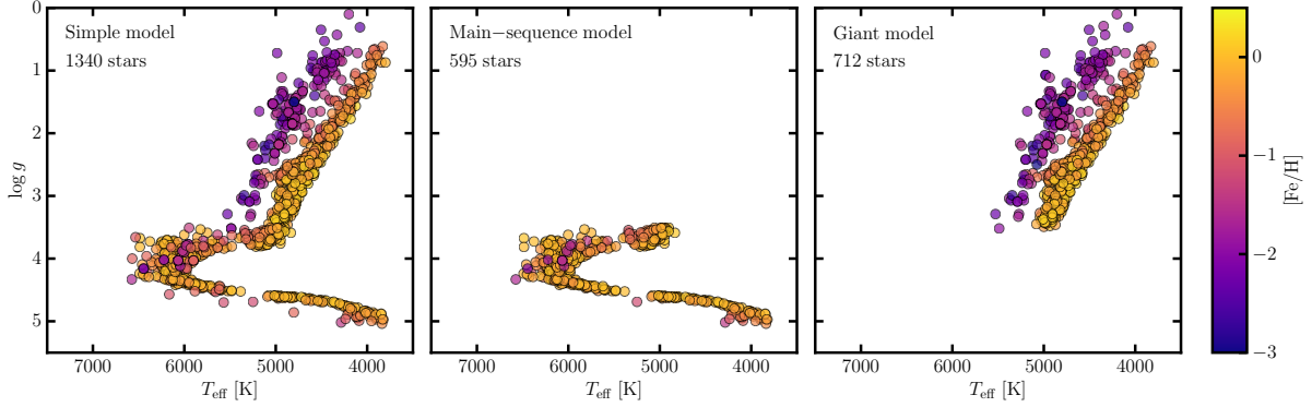
Fig. 1.— Effective temperature T_{\text{eff}} and surface gravity \log g for all stars in the training sets. Stars are colored by their metallicity [\text{Fe}/\text{H}] , and the three panels show stars in the simple model (left panel; Section 3.3), the main-sequence star model (middle panel; Section 3.4), and the giant star model (right panel; Section 3.5).
